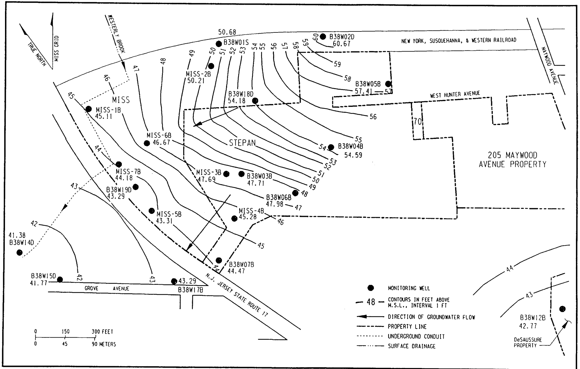
Figure 3-24 Contour Map Showing Water Level Elevations in Bedrock at MISS, September 4, 1991
