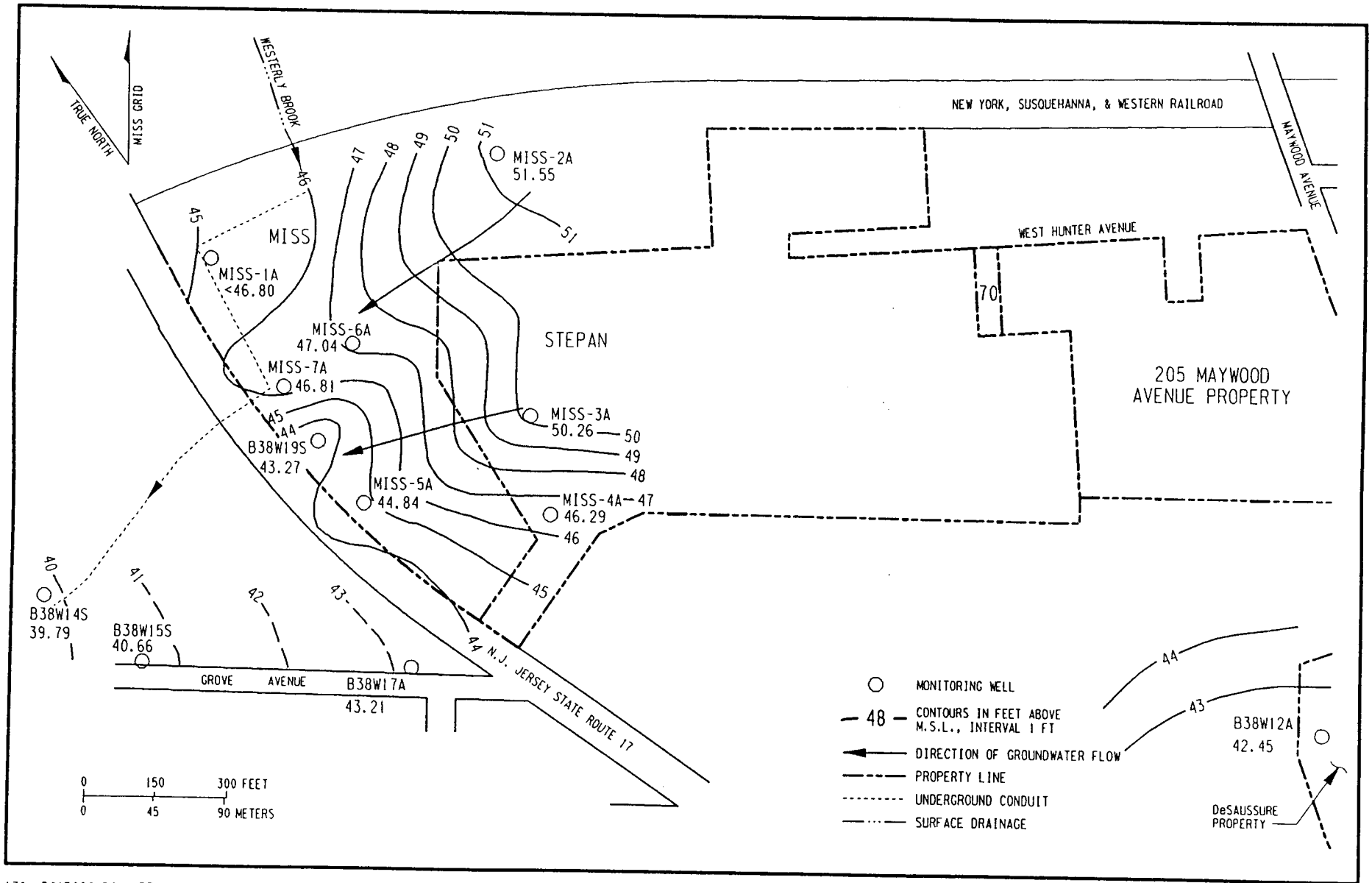
Figure 3-23 Contour Map Showing Water Level Elevations in Unconsolidated Sediments at MISS, September 4, 1991
