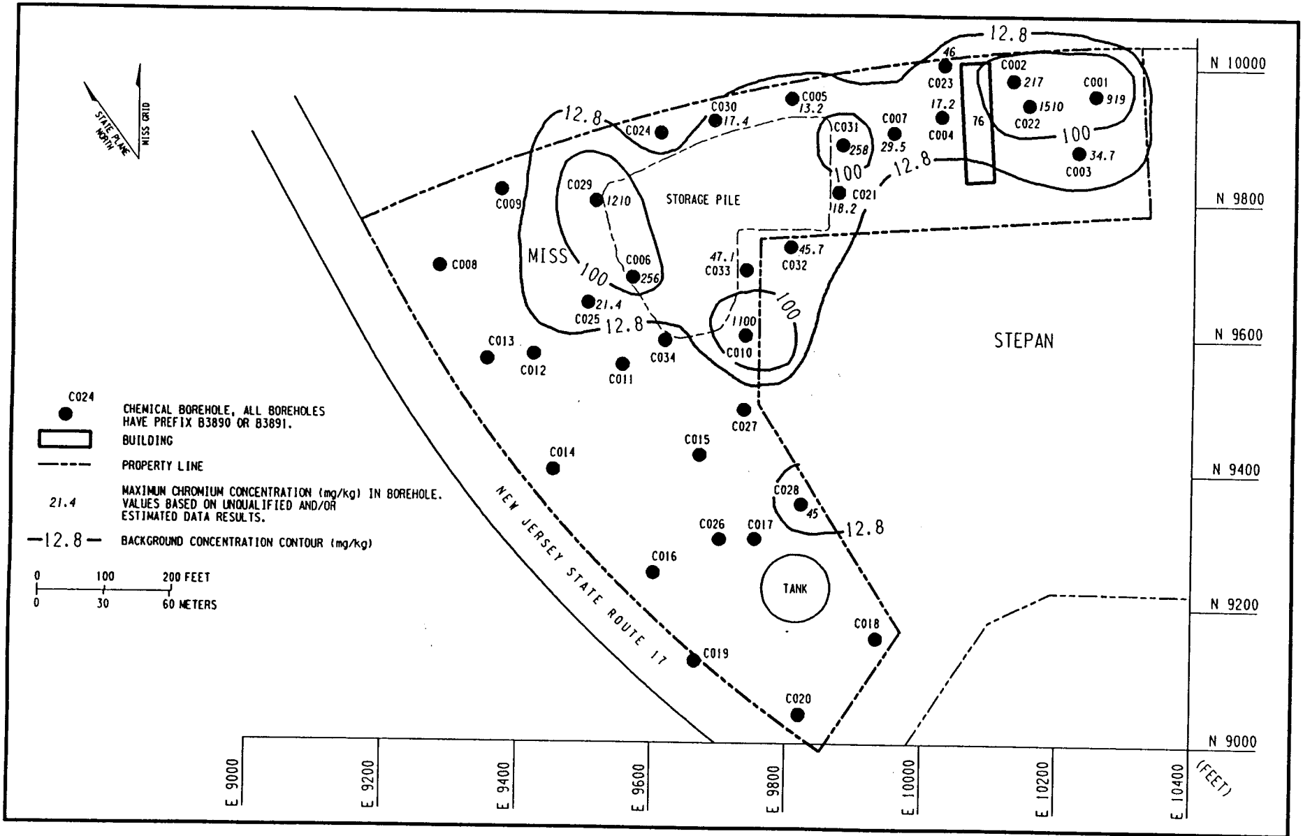
Figure 4-30 Total Chromium in Soil at MISS
