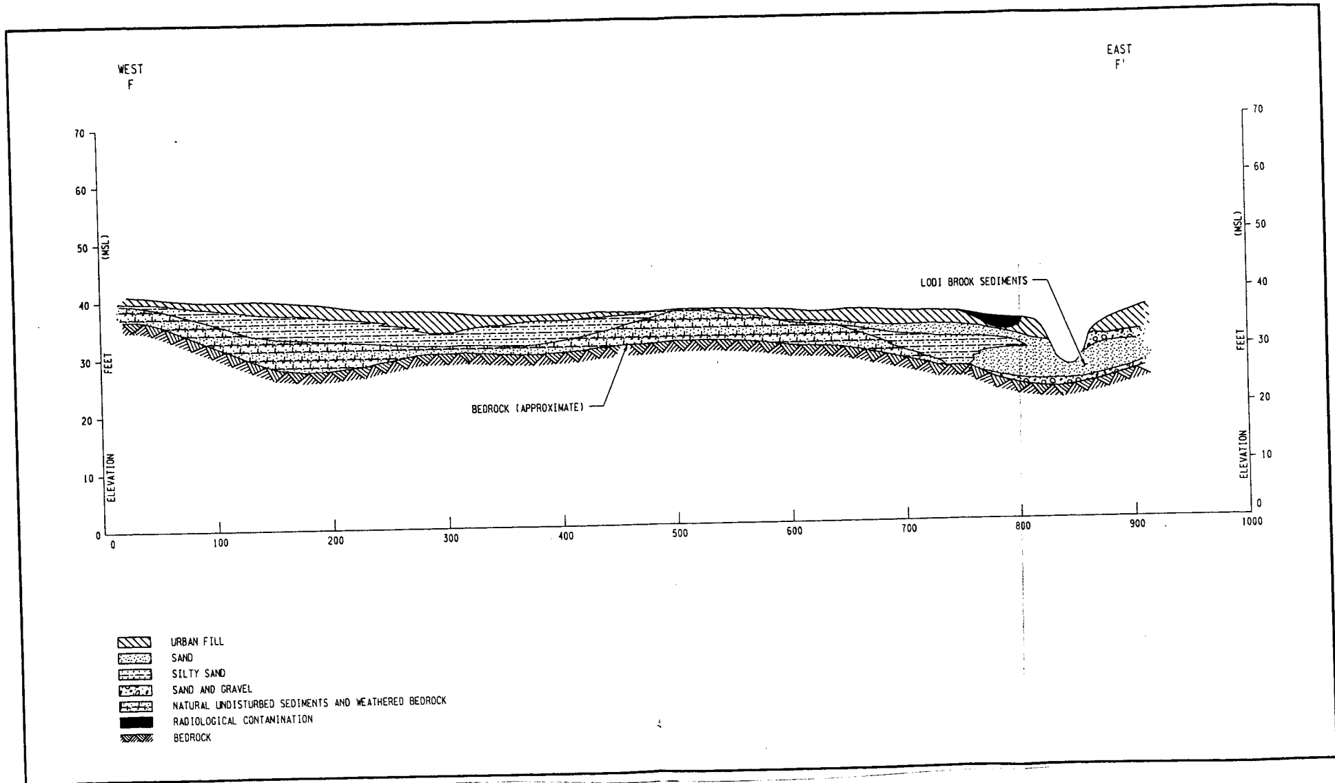
Figure 3-18 Diagrammatic Cross Section F-F' of Lodi Study Area
