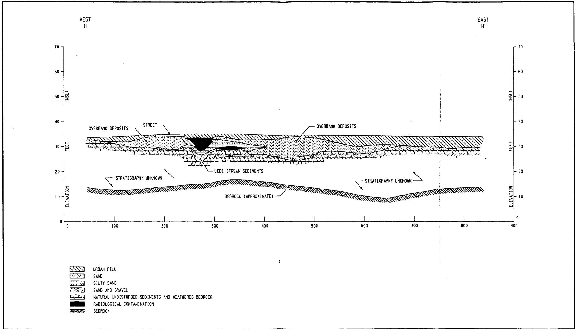
Figure 3-20 Diagrammatic Cross Section H-H' of Lodi Study Area
