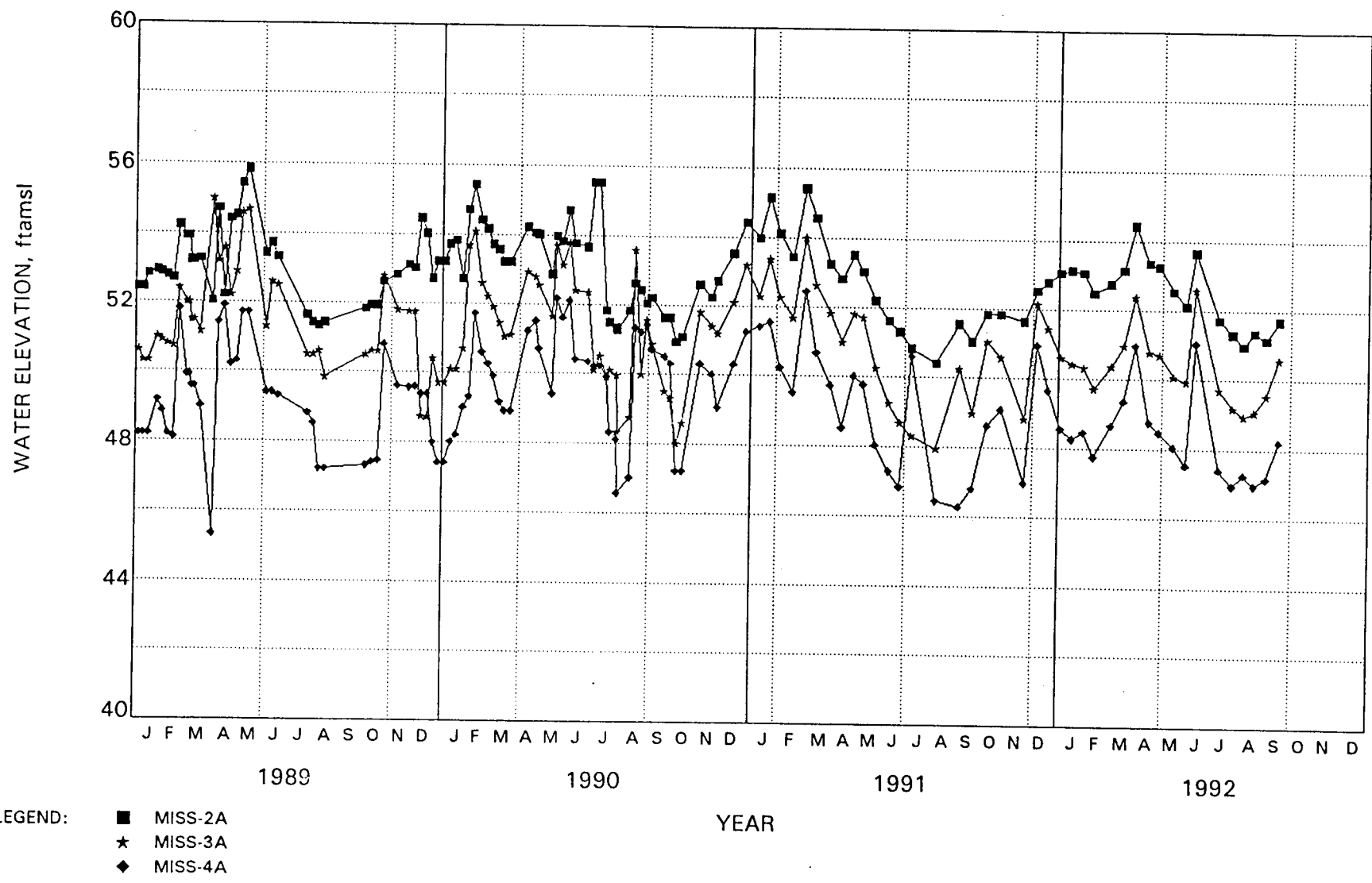
Figure 3-21 Hydrographs, Wells MISS-2A, MISS-3A, and MISS-4A
