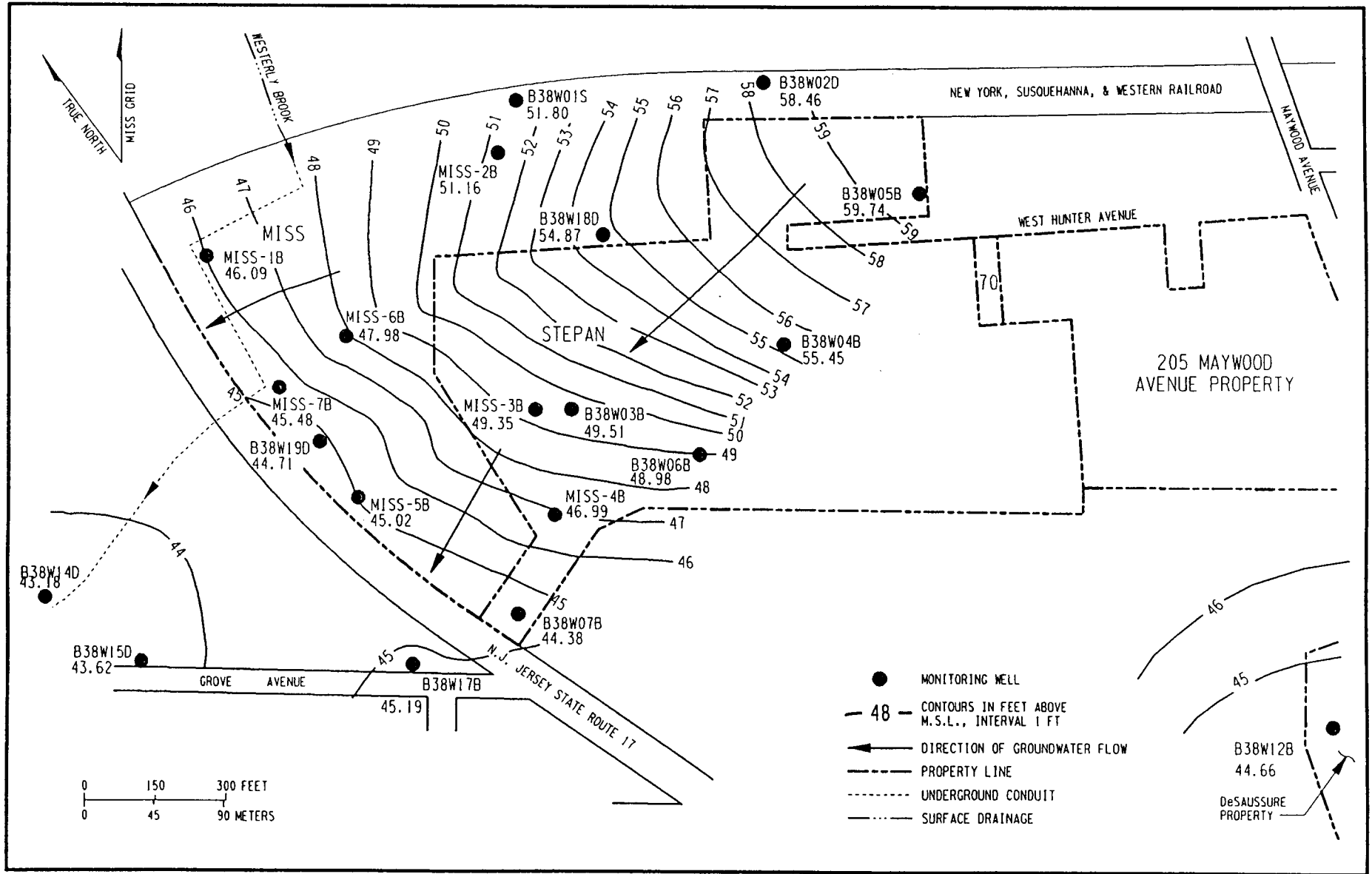
Figure 3-26 Contour Map Showing Water Level Elevations in Bedrock at MISS, March 30, 1992
