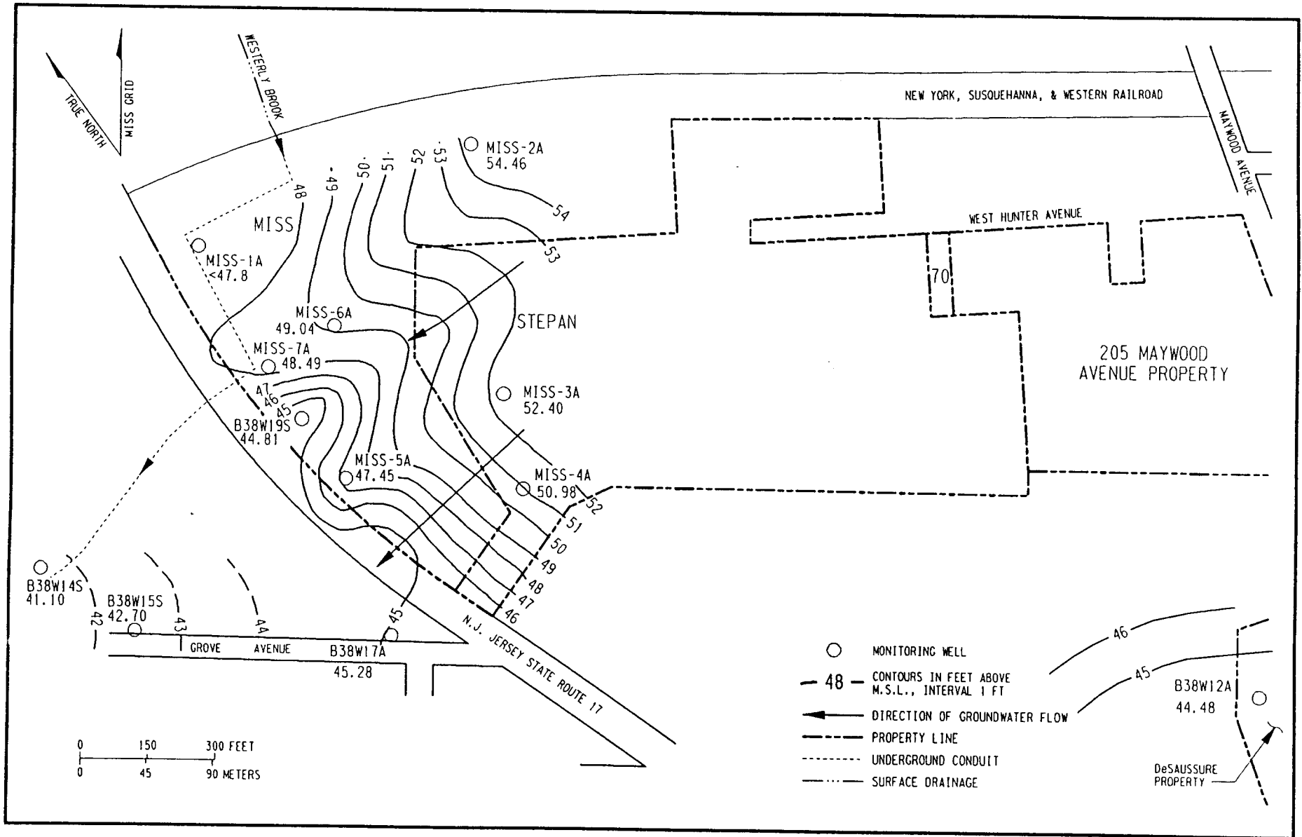
Figure 3-25 Contour Map Showing Water Level Elevations in Unconsolidated Sediments at MISS, March 30, 1992
