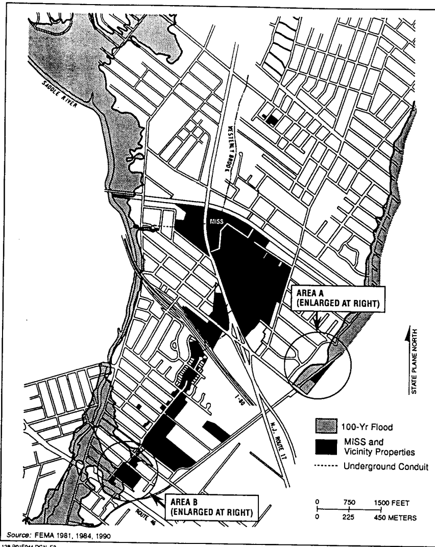
Figure 3-4 100-Year-Flood Zones in the Maywood Area
