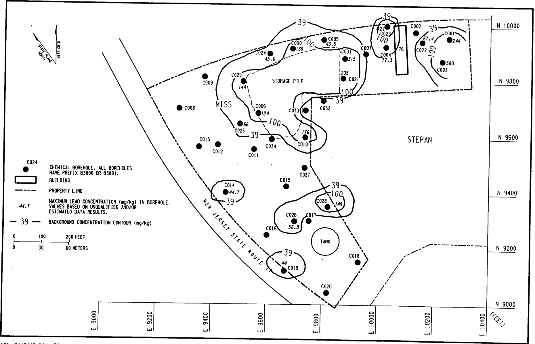
Figure 4-32 Total Lead in Soil at MISS
