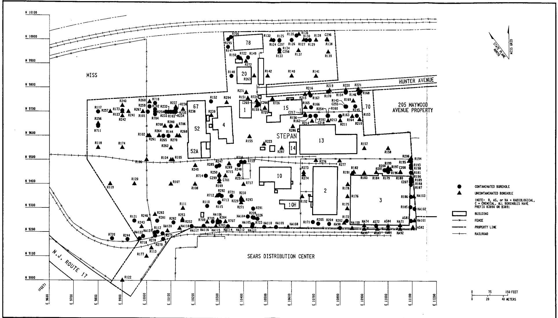
Figure 4-17 Stepan Property Borehole Locations
