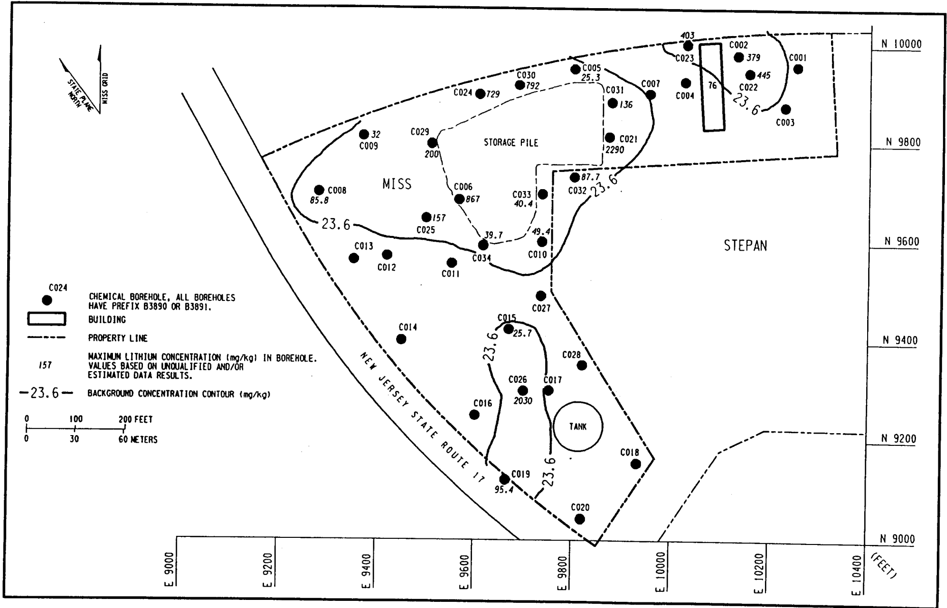
Figure 4-33 Total Lithium in Soil at MISS
