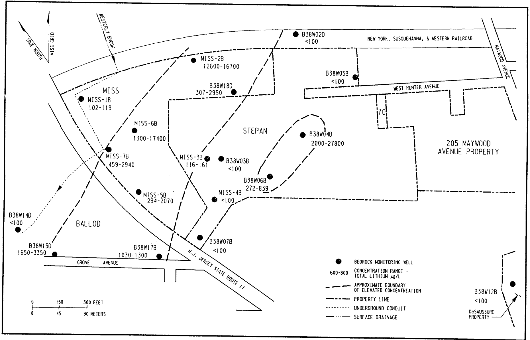
Figure 4-68 Concentration and Distribution of Lithium in Groundwater
