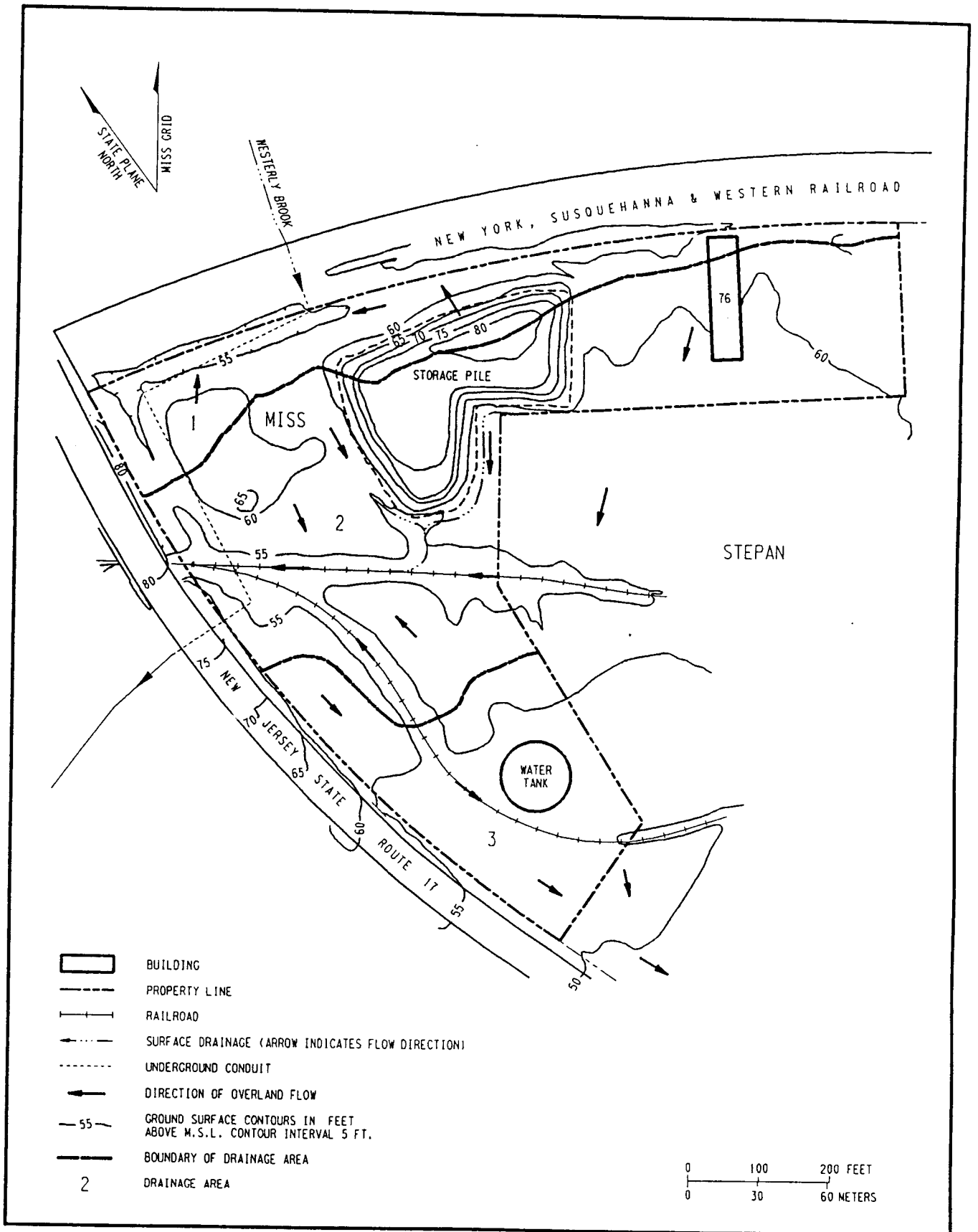
Figure 3-2 MISS Drainage Areas and Direction of Overland Flow
