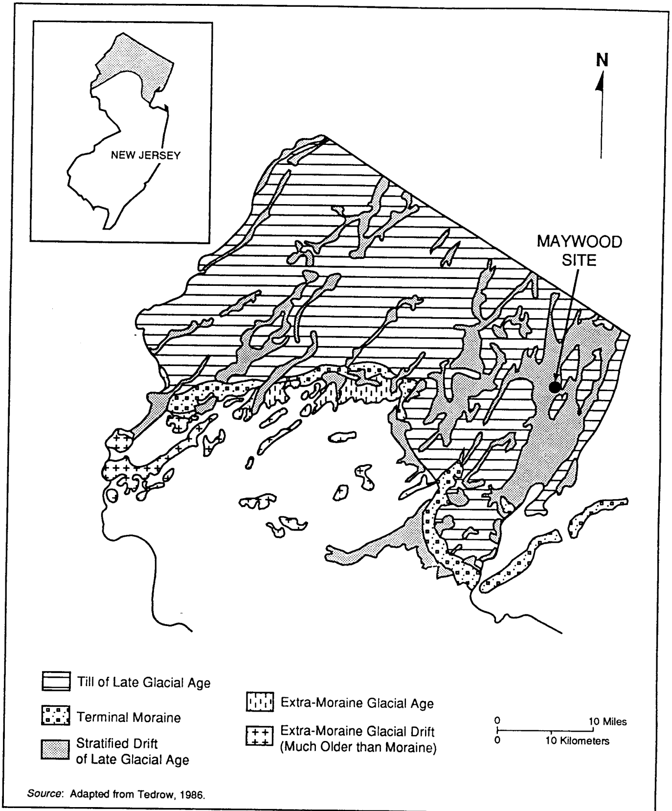
Figure 3-7 Glacial Deposits in New Jersey
