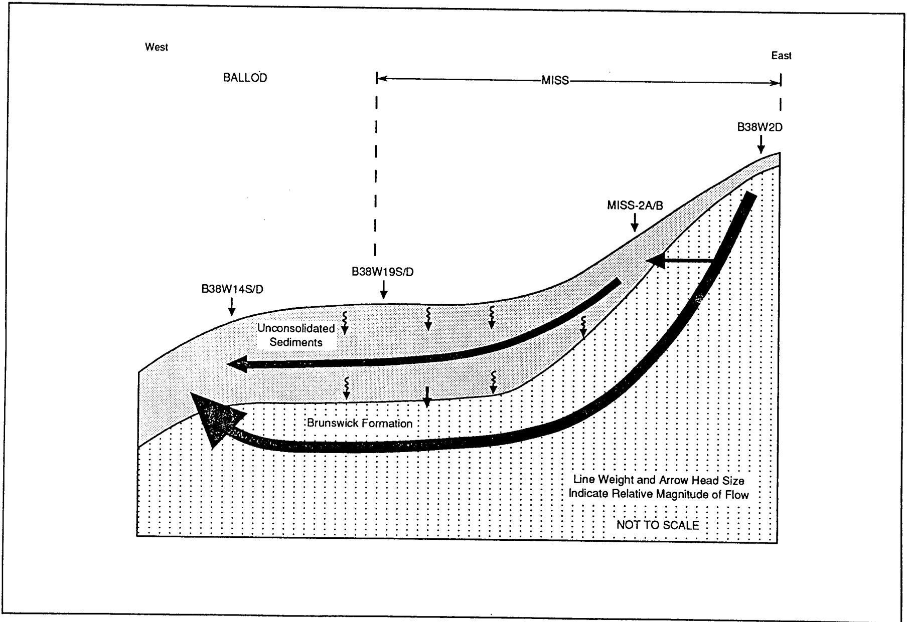
Figure 3-27 Conceptual Groundwater Flow System at MISS
