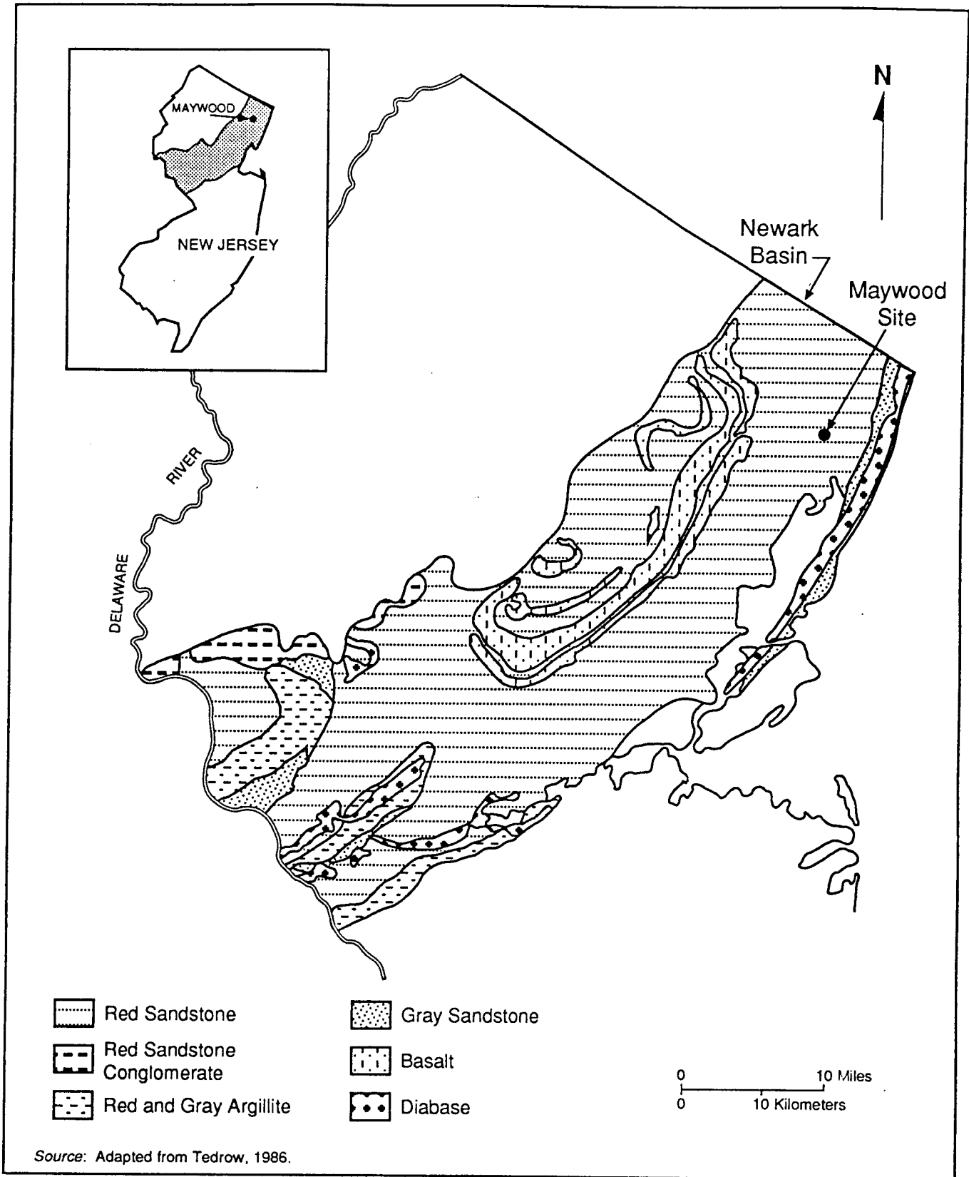
Figure 3-5 Distribution of Triassic/Jurassic Formations in the Newark Basin
