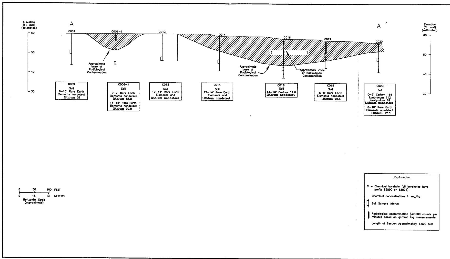
Figure 4-36 MISS Cross Section A-A'
