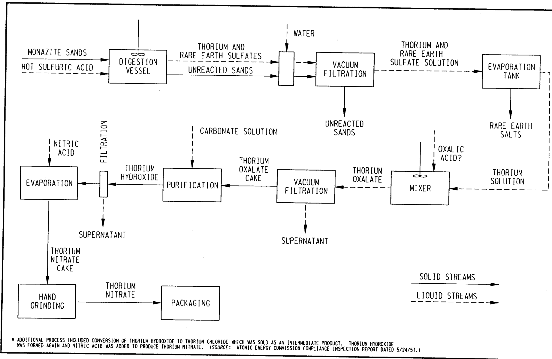
Figure 1-5 Process Possibly Used to Produce Mantle-Grade Thorium Nitrate at MCW
