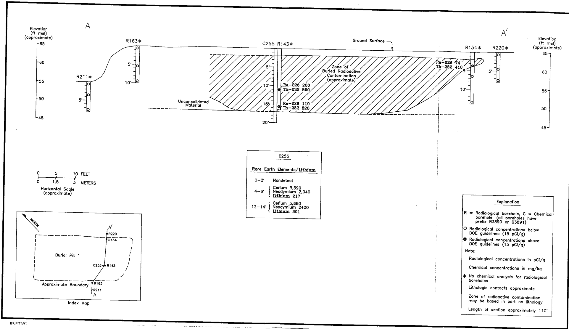
Figure 4-21 Stepan Burial Pit 1, Cross Section A-A'
