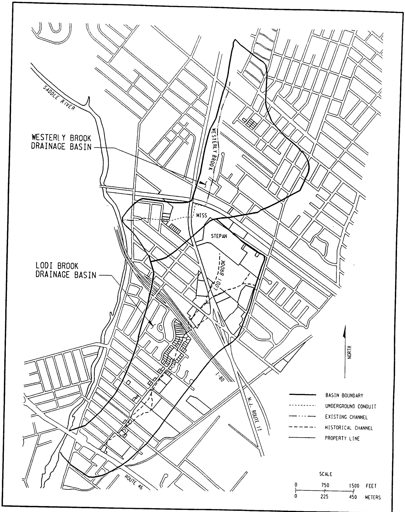
Figure 3-1 Drainage Basins in the Maywood and Lodi Areas
