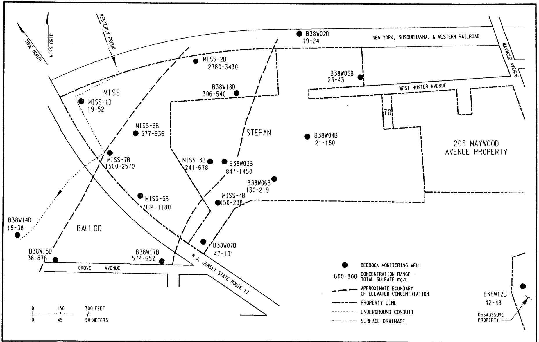
Figure 4-67 Concentration and Distribution of Sulfate in Groundwater
