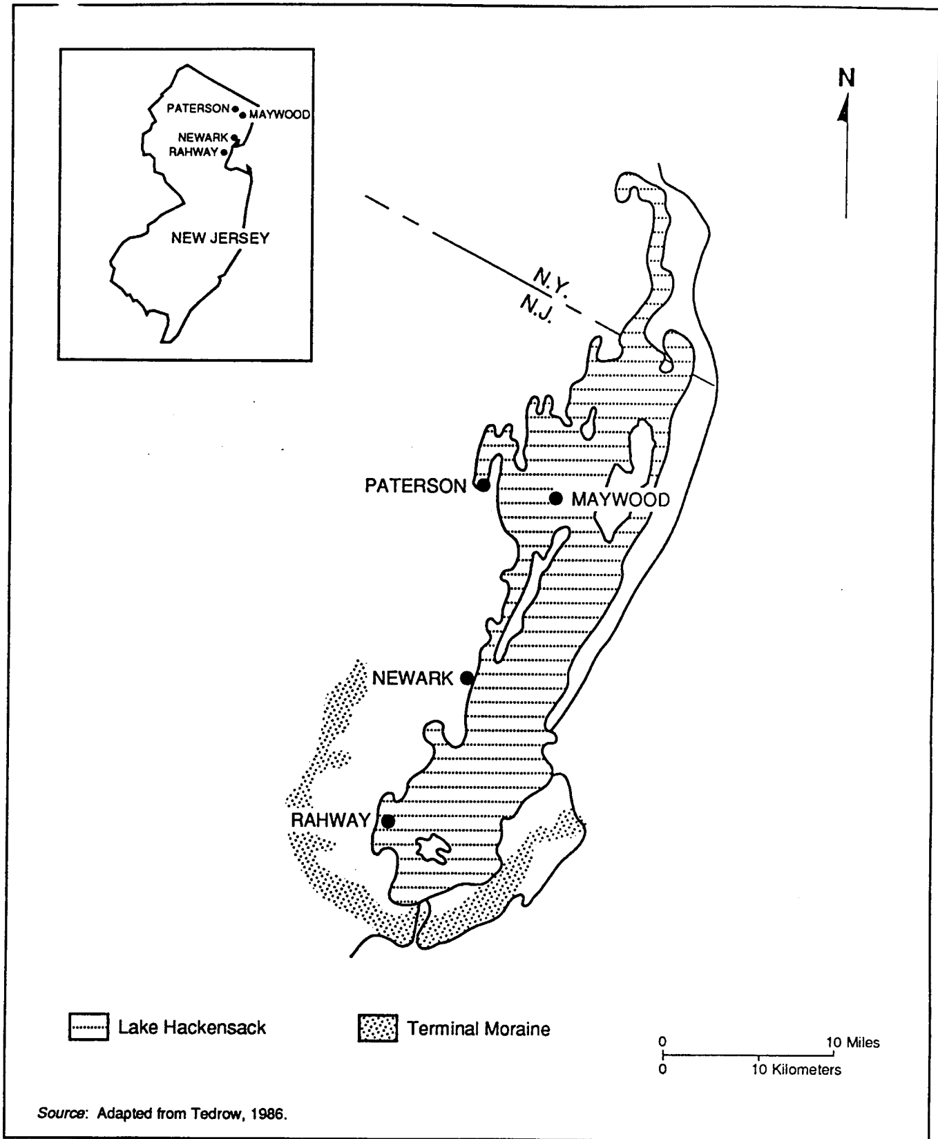
Figure 3-8 Preglacial Lake Hackensack
