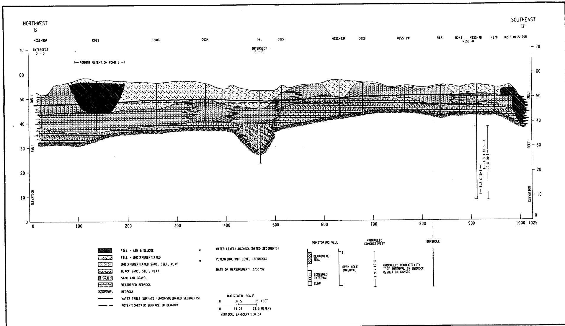
Figure 3-13 Hydrogeologic Cross Section B-B' at MISS
