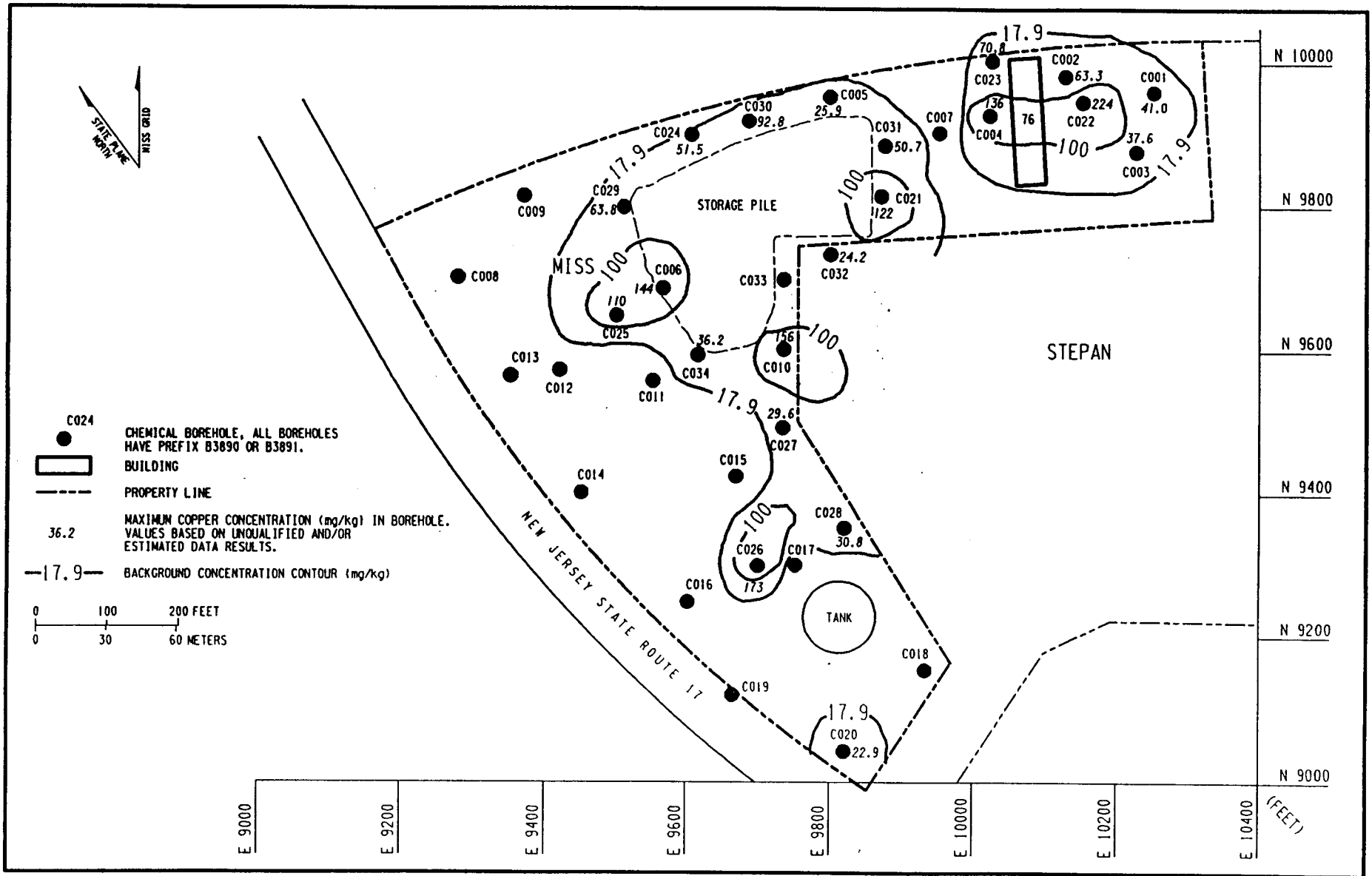
Figure 4-31 Total Copper in Soil at MISS
