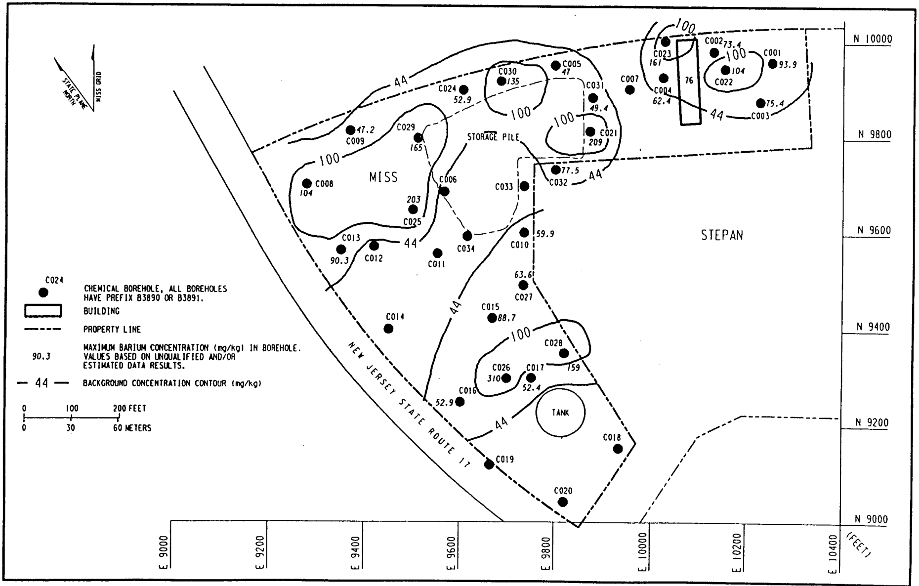
Figure 4-29 Total Barium in Soil at MISS
