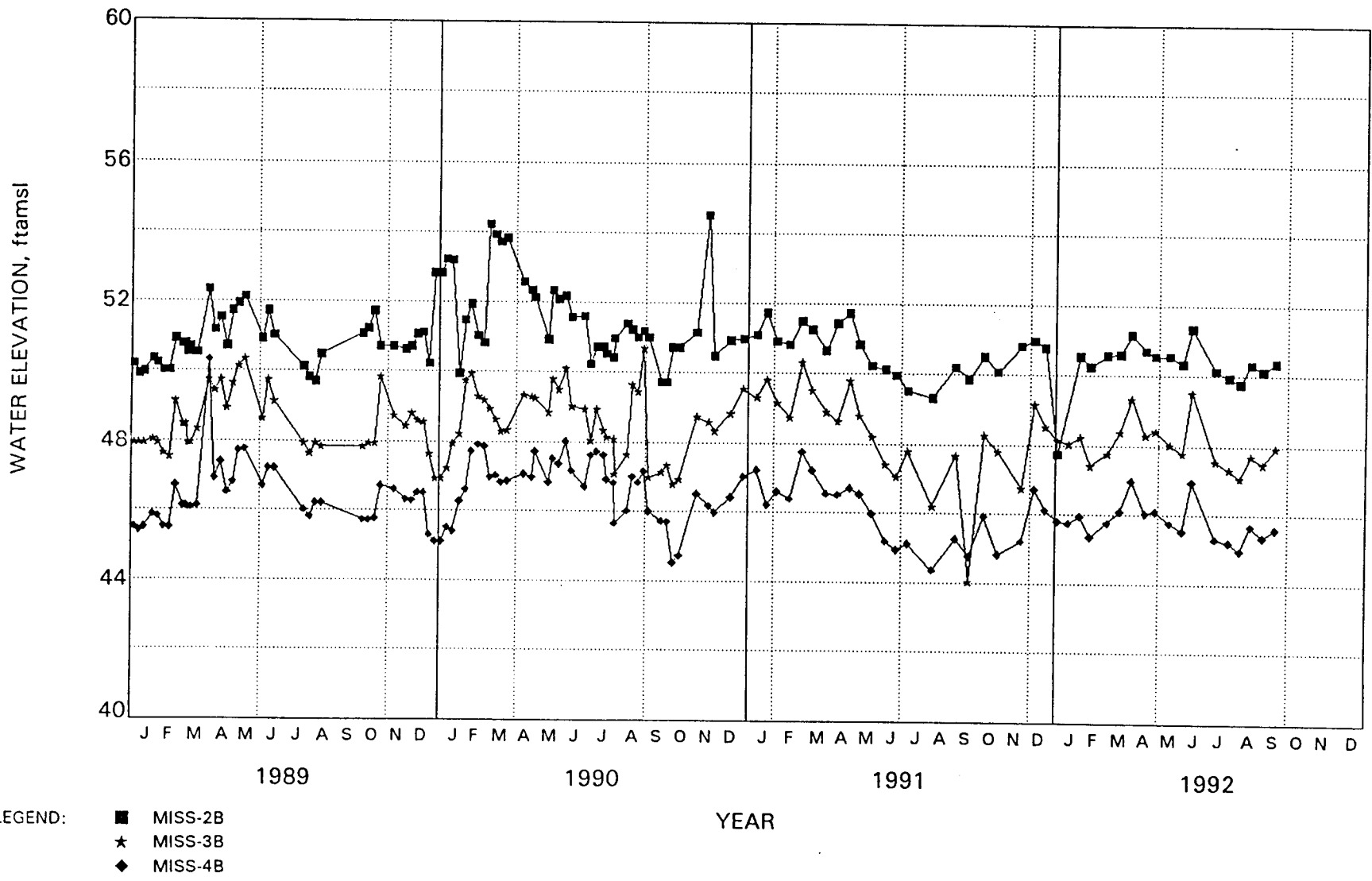
Figure 3-22 Hydrographs, Wells MISS-2B, MISS-3B, and MISS-4B
