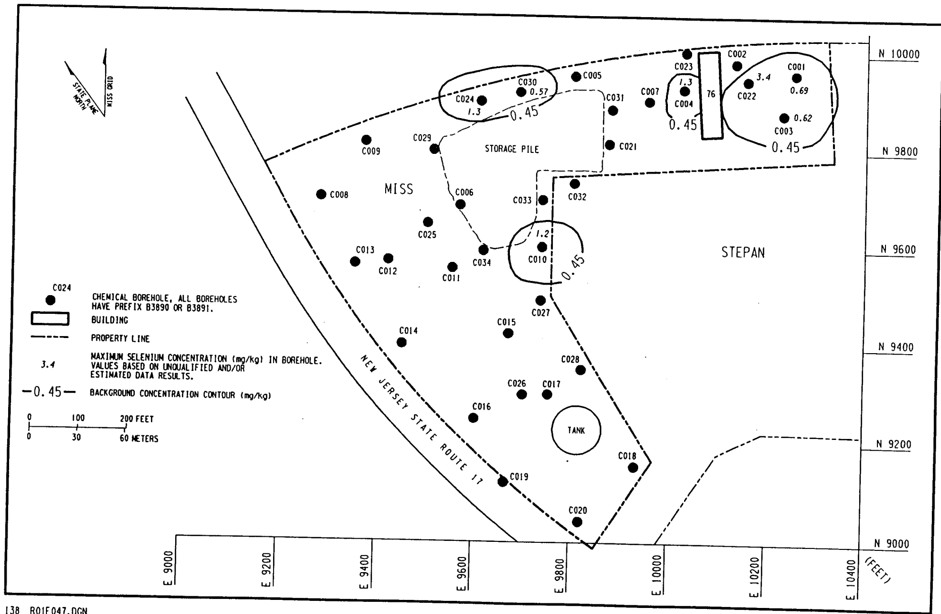
Figure 4-34 Total Selenium in Soil at MISS
