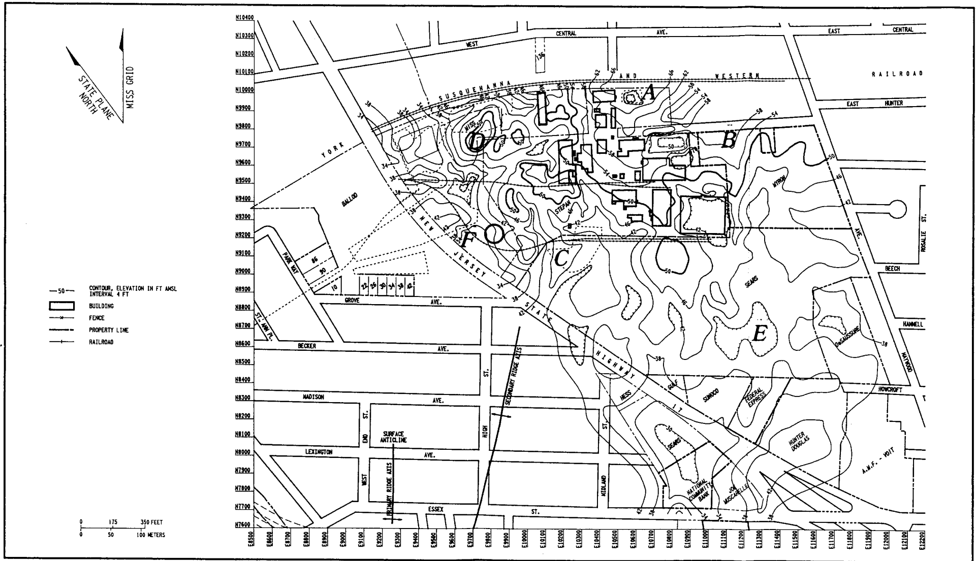
Figure 3-10 Contour Map of the Top of Bedrock in the Maywood Area
