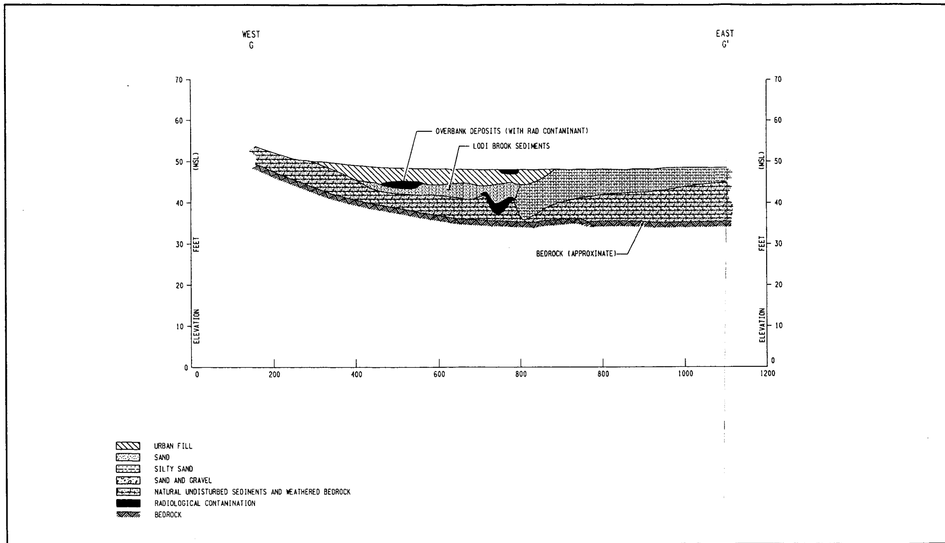
Figure 3-19 Diagrammatic Cross Section G-G' of Lodi Study Area
