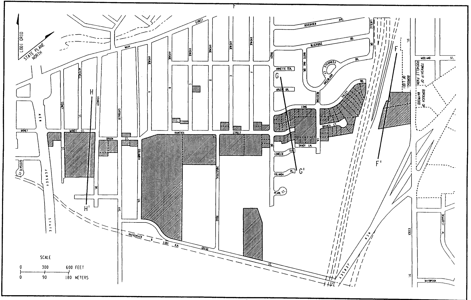
Figure 3-17 Approximate Locations of Diagrammatic Cross Sections of the Lodi Study Area
