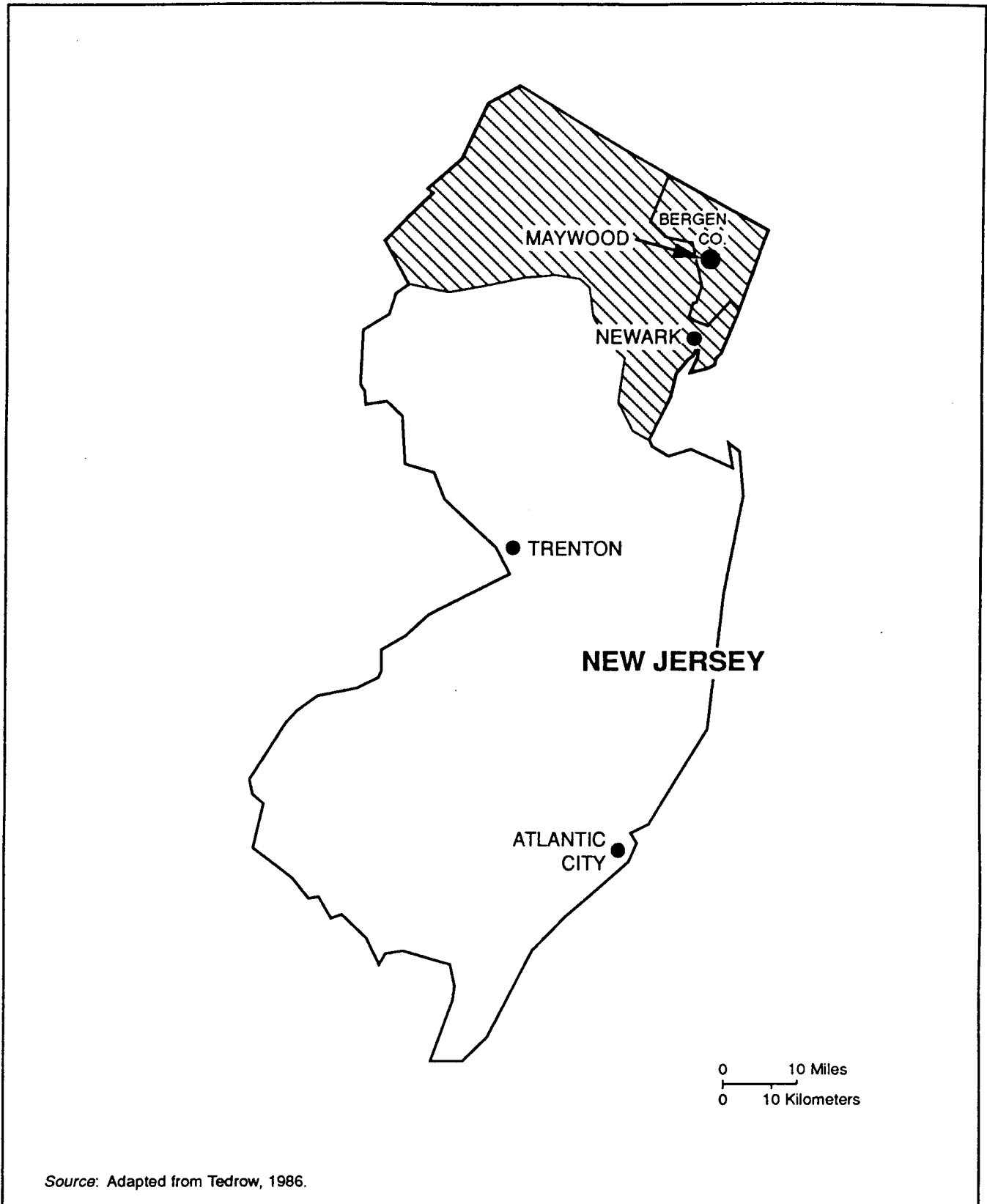
Figure 3-6 Ice Cover in New Jersey During Wisconsin Glacial Maximum
