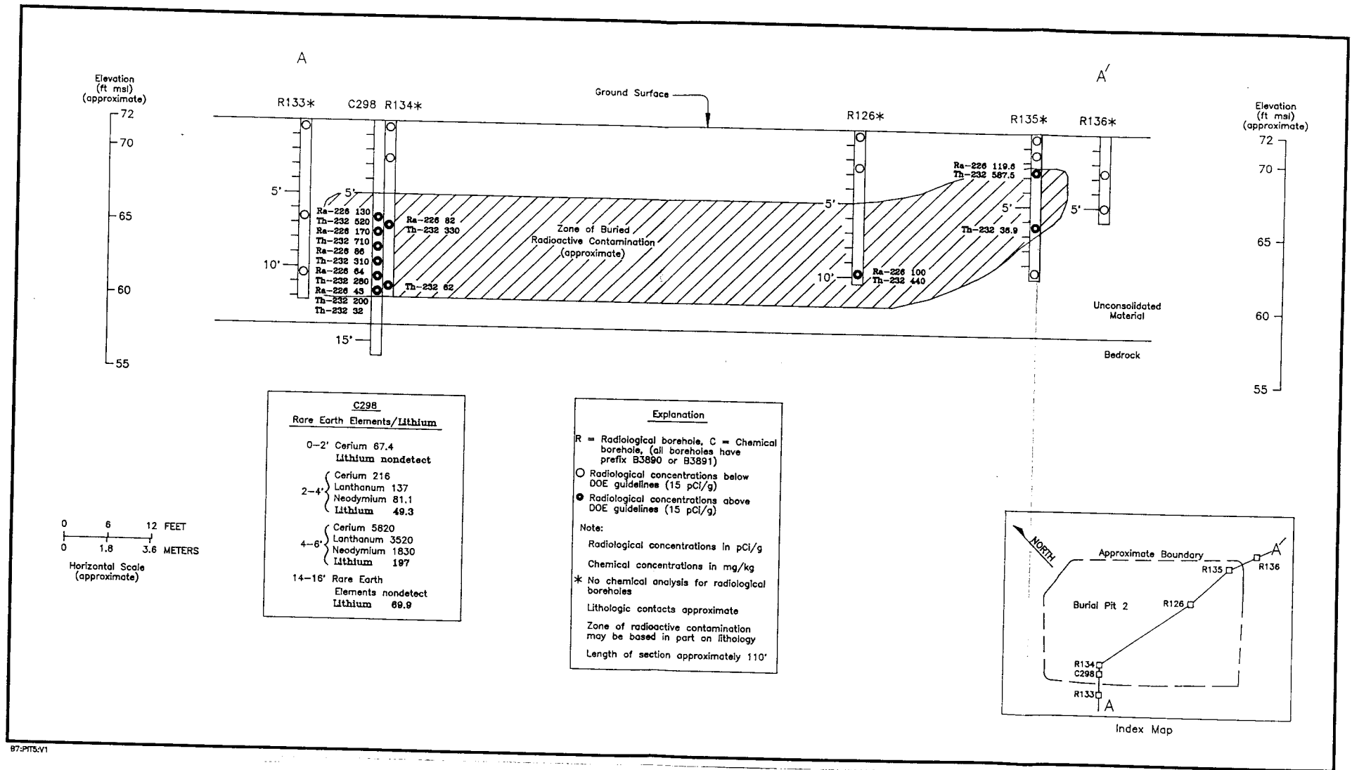
Figure 4-23 Stepan Burial Pit 2, Cross Section A-A'
