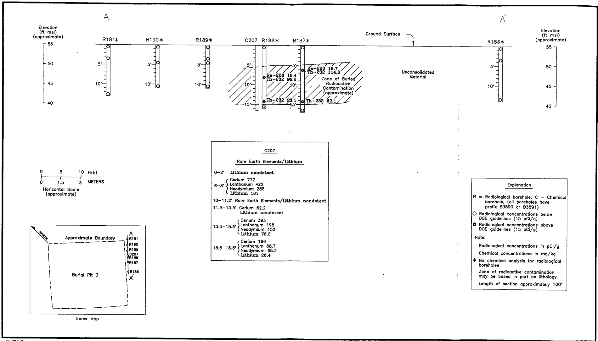
Figure 4-25 Stepan Burial Pit 3, Cross Section A-A'
