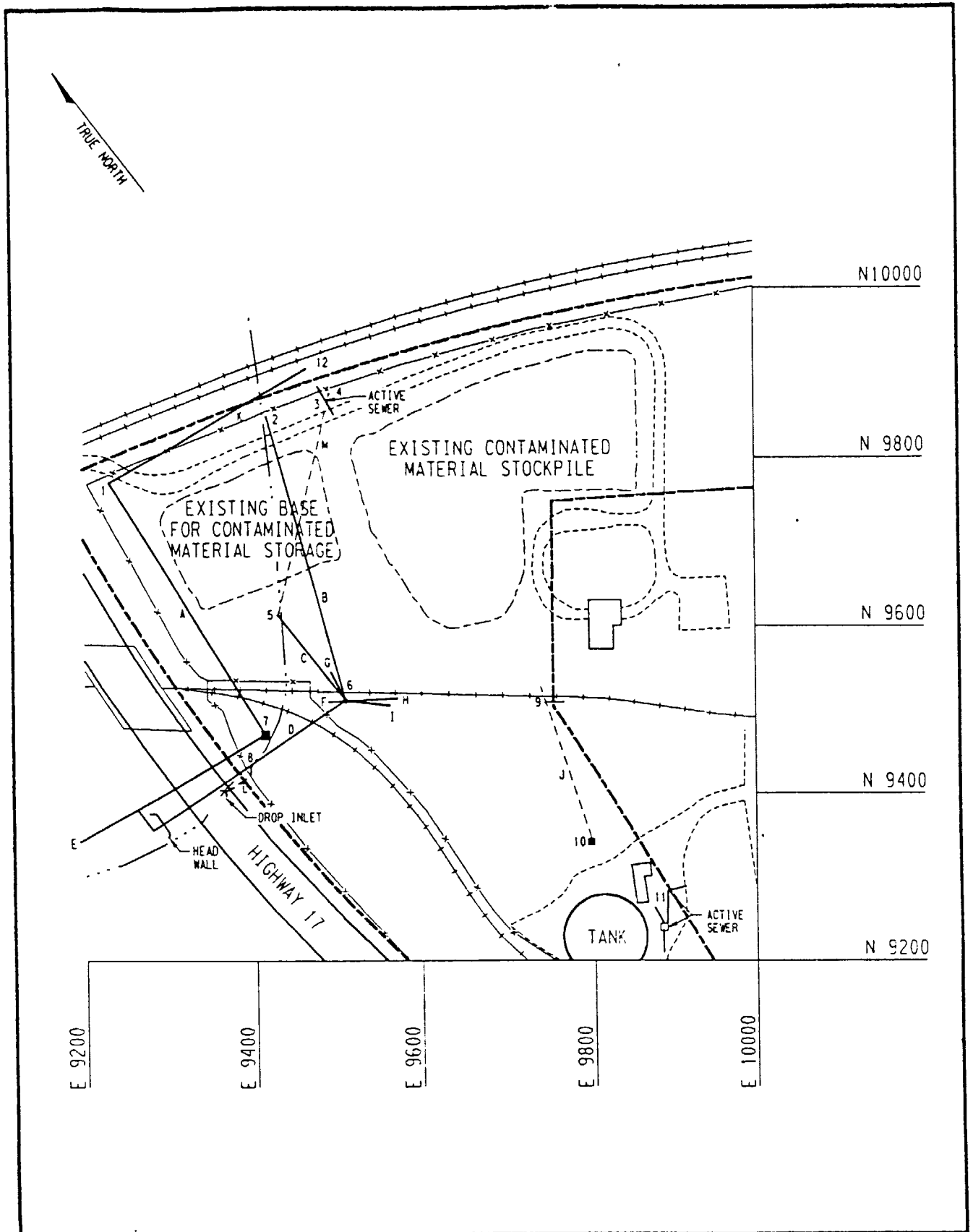
FIGURE 1 SEWER/DRAINAGE LINES AT MISS
