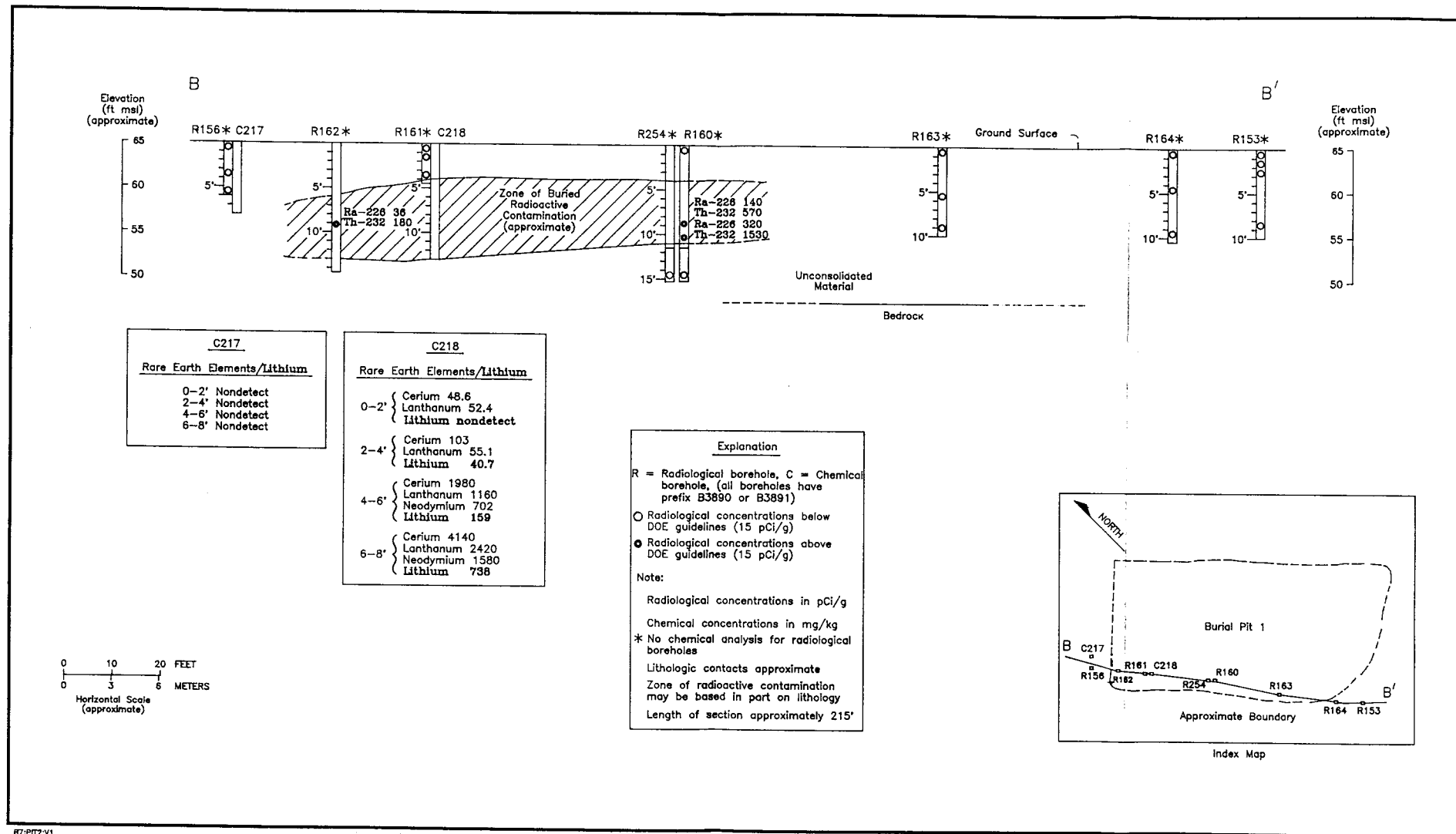
Figure 4-22 Stepan Burial Pit 1, Cross Section B-B'
