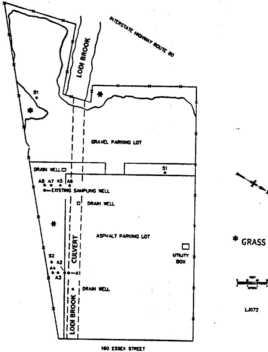
Fig. 2. Diagram showing locations of soil samples taken at 160 Essex Street, Lodi, New Jersey (LJ072).
