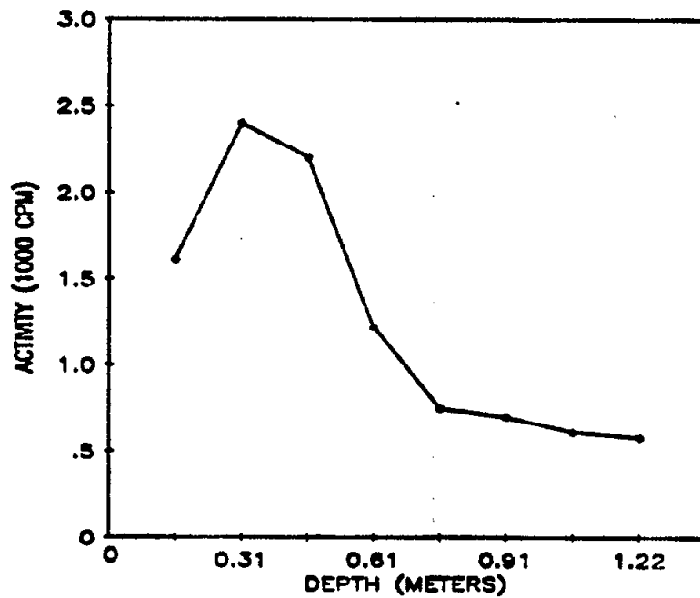
Fig. 9. Gamma profile for auger hole 7 (LJ072A7) at 160 Essex Street, Lodi, New Jersey.
