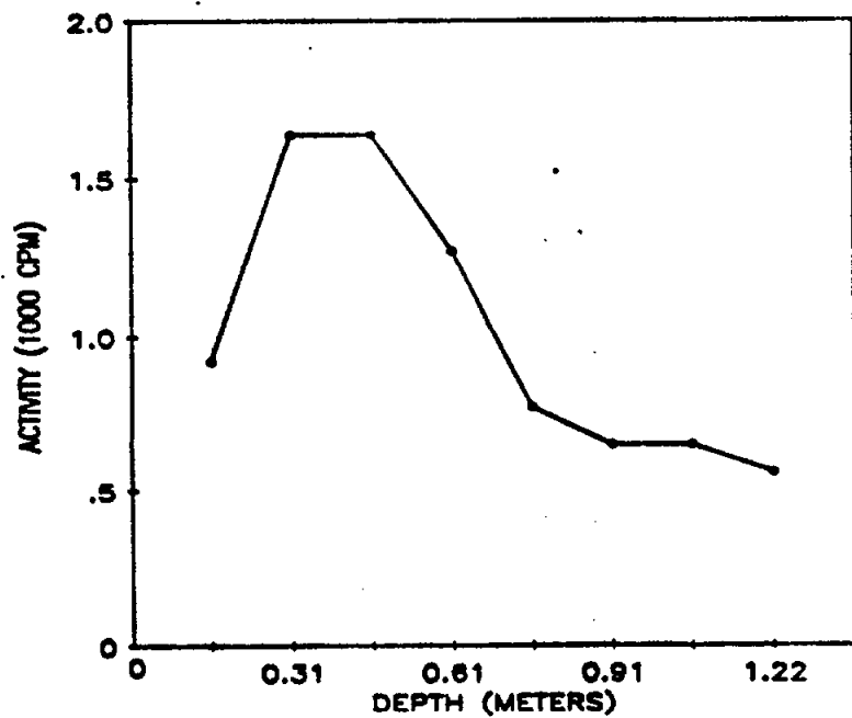
Fig. 8. Gamma profile for auger hole 6 (LJ072A6) at 160 Essex Street, Lodi, New Jersey.
