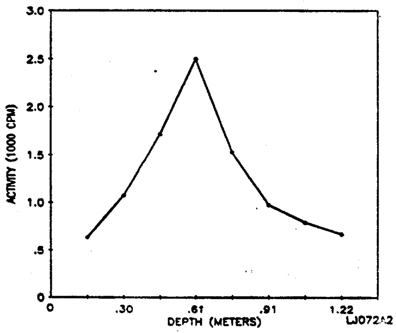
Fig. 4. Gamma profile for auger hole 2 (LJ072A2) at 160 Essex Street, Lodi, New Jersey.
