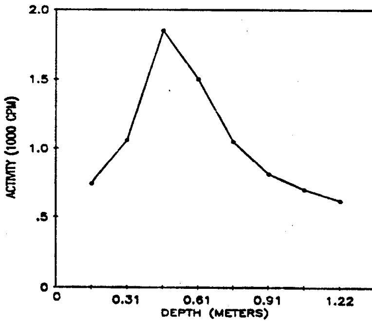
Fig. 5. Gamma profile for auger hole 3 (LJ072A3) at 160 Essex Street, Lodi, New Jersey.
