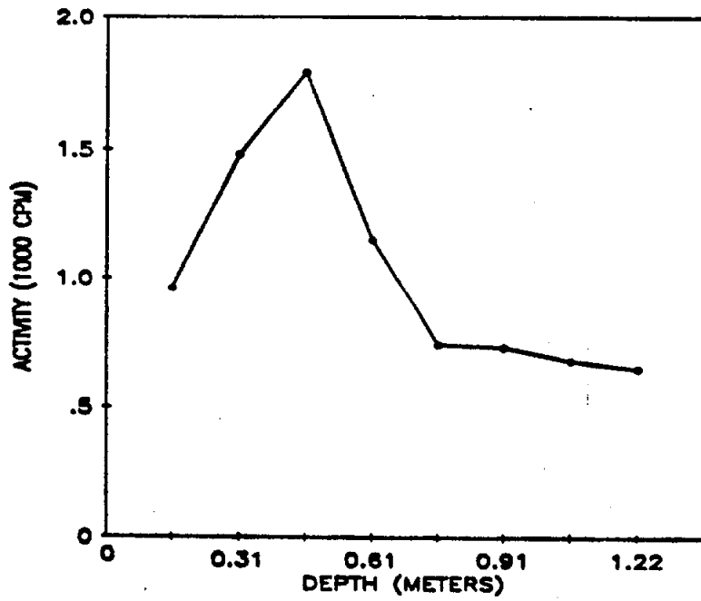
Fig. 10. Gamma profile for auger hole 8 (LJ072A8) at 160 Essex Street, Lodi, New Jersey.
