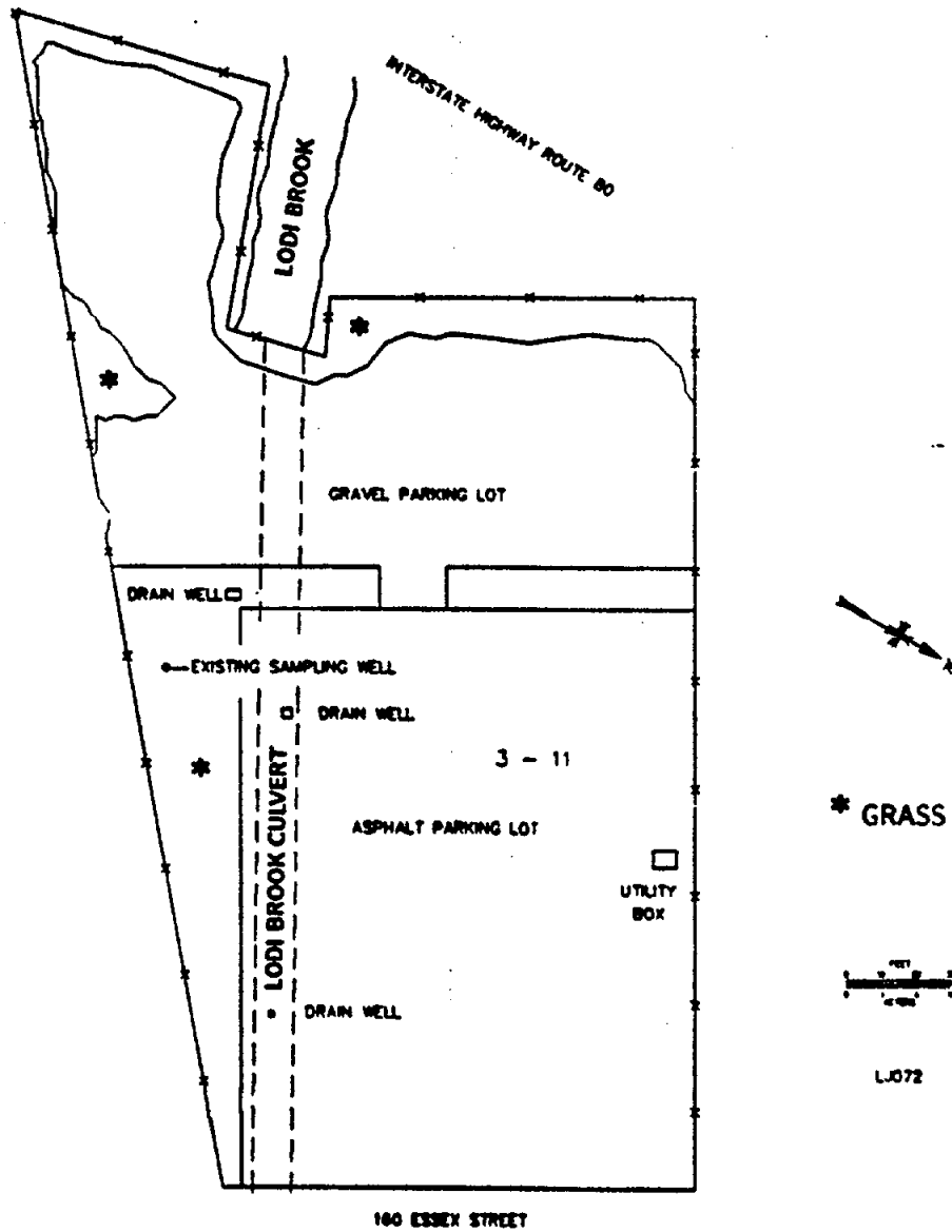
Fig. 1. Gamma radiation levels ( \mu\text{R}/\text{h} ) measured on the surface at 160 Essex Street, Lodi, New Jersey (LJ072).
