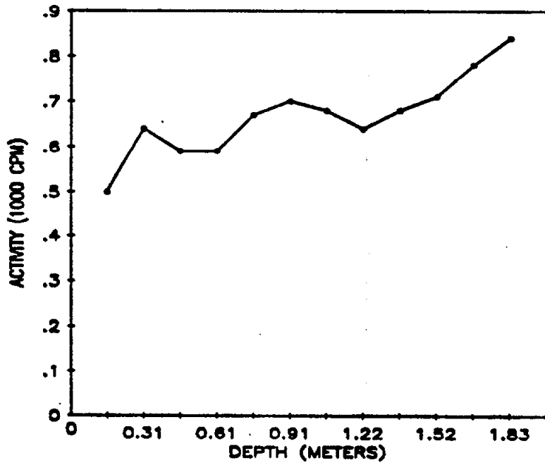
Fig. 6. Gamma profile for auger hole 4 (LJ072A4) at 160 Essex Street, Lodi, New Jersey.
