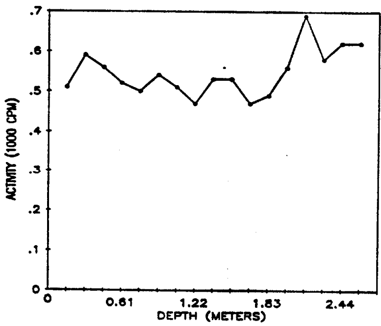
Fig. 3. Gamma profile for auger hole 1 (LJ072A1) at 160 Essex Street, Lodi, New Jersey.
