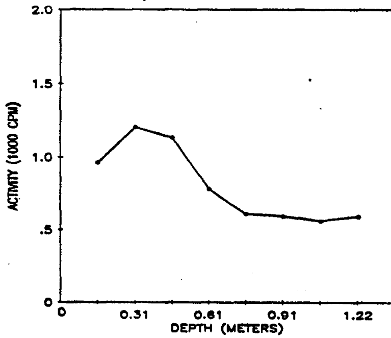
Fig. 7. Gamma profile for auger hole 5 (LJ072A5) at 160 Essex Street, Lodi, New Jersey.
