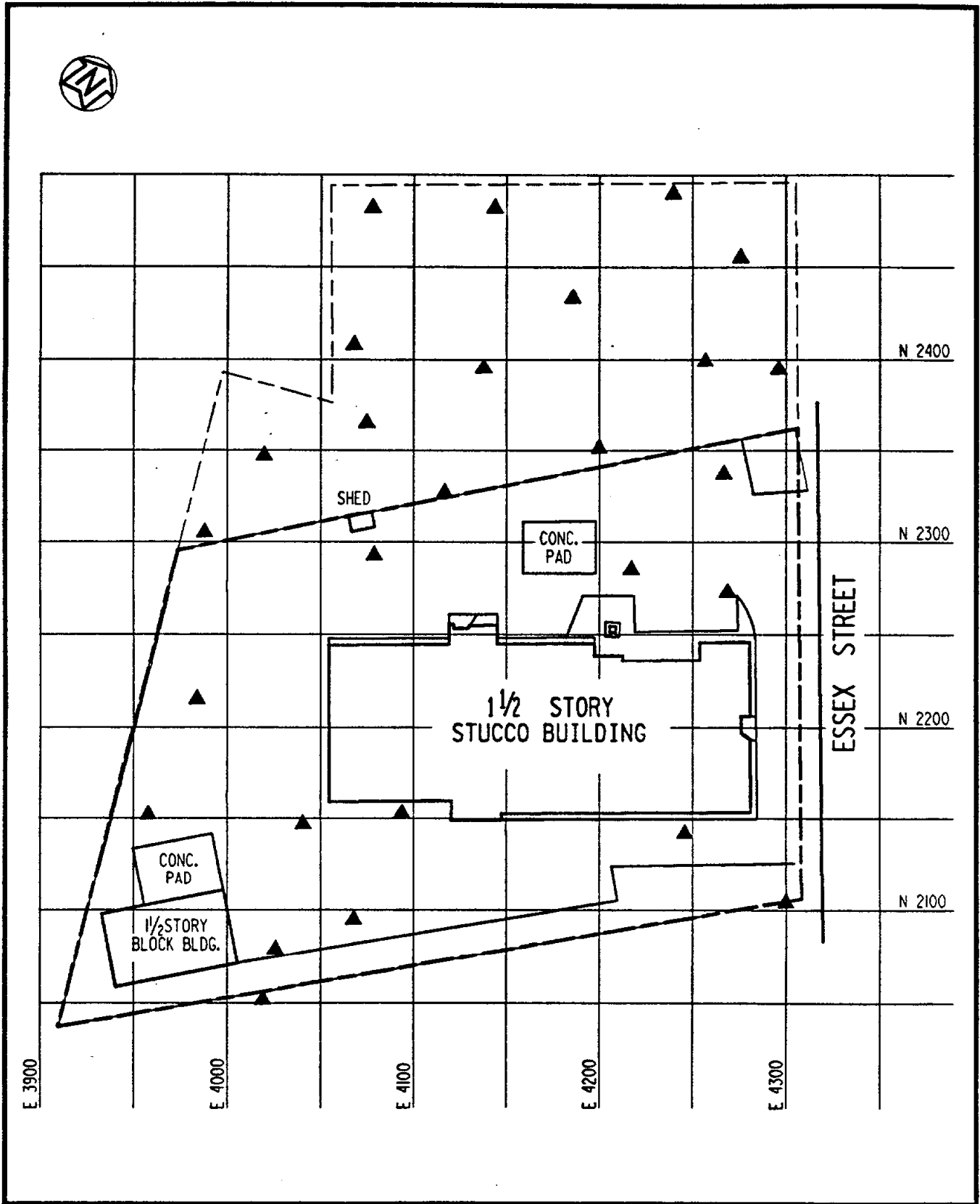
FIGURE 4-2 SURFACE AND SUBSURFACE SOIL SAMPLING LOCATIONS AT 160 AND 174 ESSEX STREET
