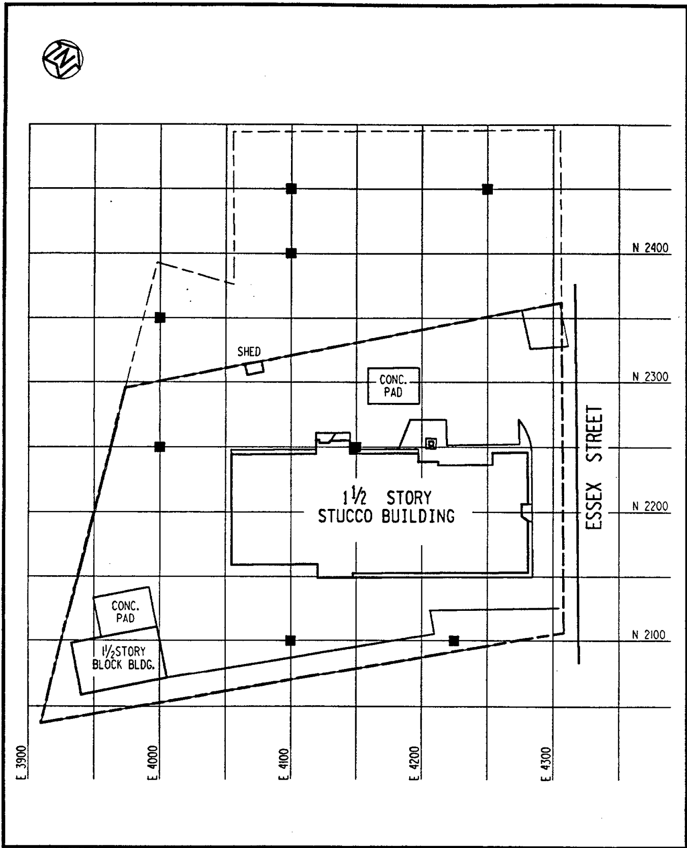
FIGURE 4-3 GAMMA EXPOSURE RATE MEASUREMENT LOCATIONS AT 160 AND 174 ESSEX STREET
