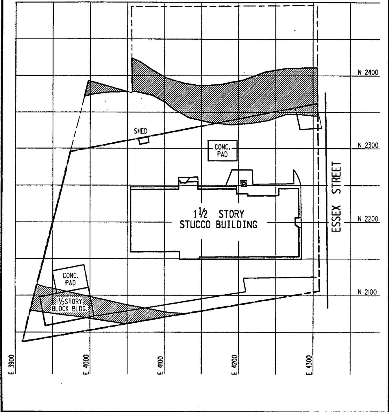
FIGURE 5-1 AREAS OF SUBSURFACE CONTAMINATION AT 160 AND 174 ESSEX STREET
