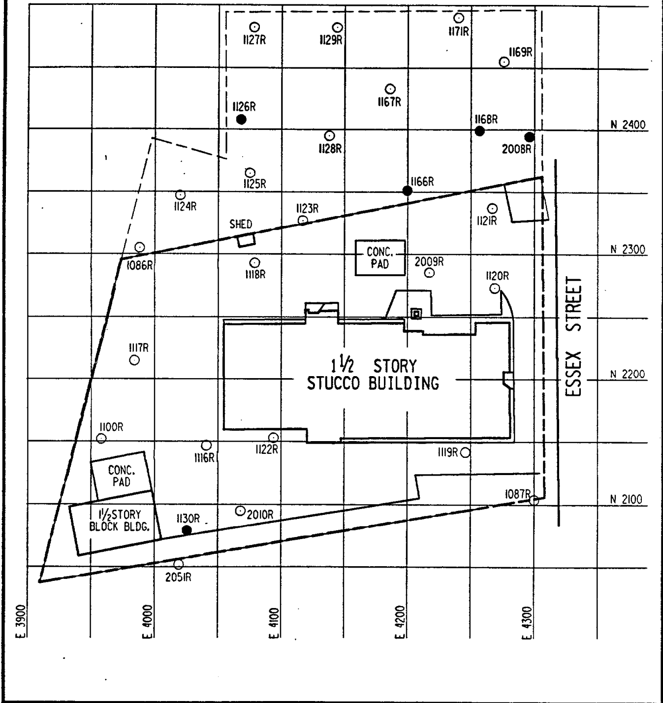
FIGURE 4-1 BOREHOLE LOCATIONS AT 160 AND 174 ESSEX STREET
