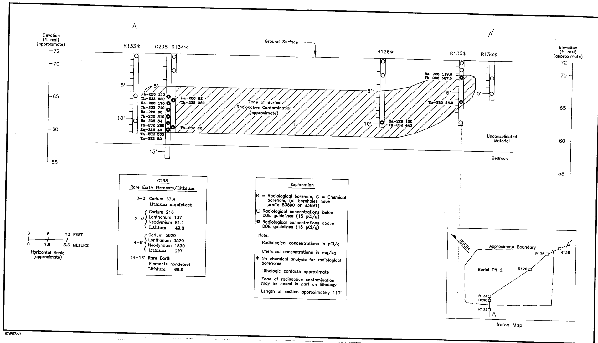
Figure 4-23 Stepan Burial Pit 2, Cross Section A-A'
