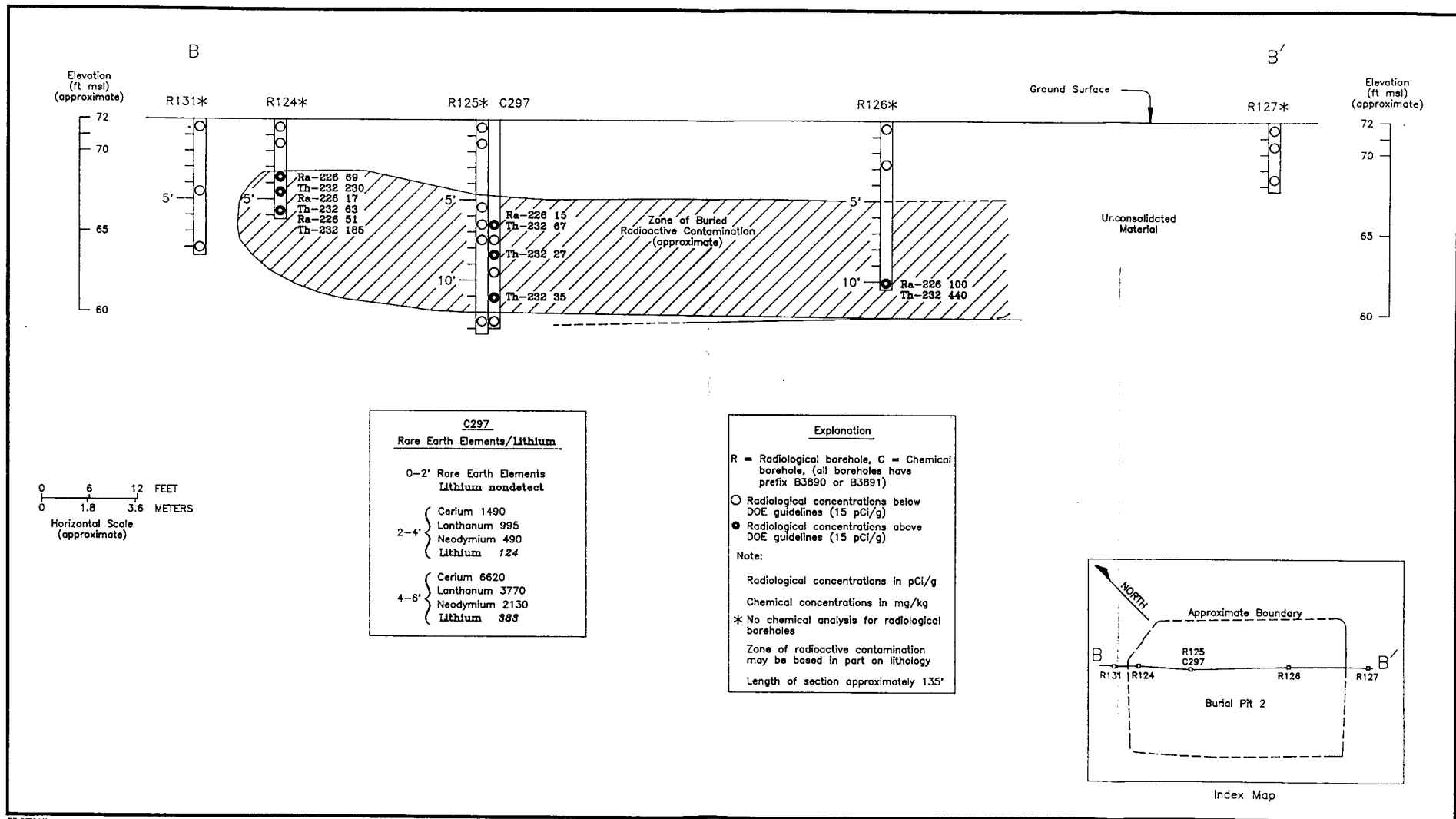
Figure 4-24 Stepan Burial Pit 2, Cross Section B-B'
