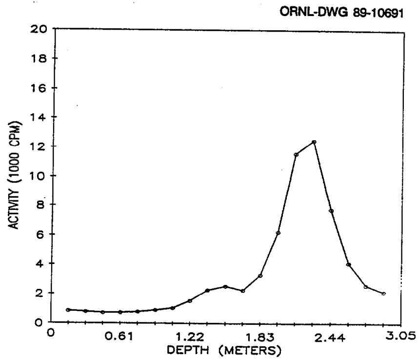
Fig. 10. Gamma profile for auger hole 24 (LJ061A24) at 80 Industrial Road, Lodi, New Jersey.
