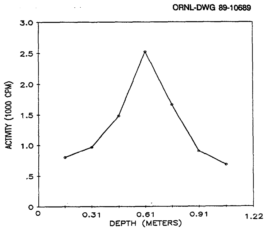
Fig. 8. Gamma profile for auger hole 9 (LJ061A9) at 80 Industrial Road, Lodi, New Jersey.
