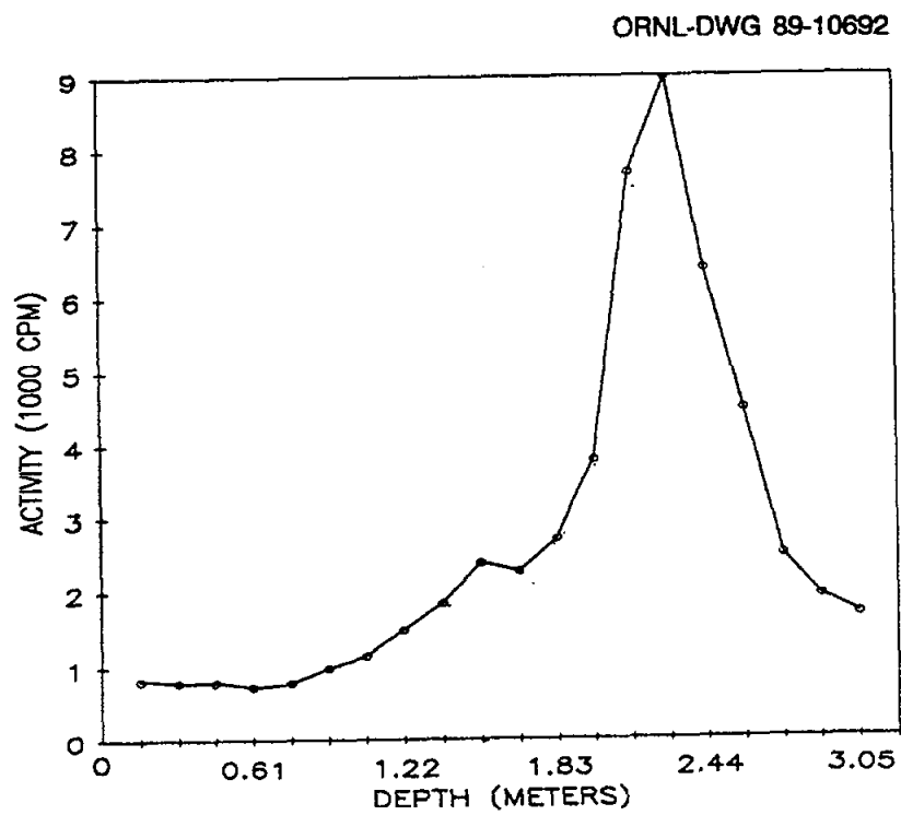
Fig. 11. Gamma profile for auger hole 25 (LJ061A25) at 80 Industrial Road, Lodi, New Jersey.
