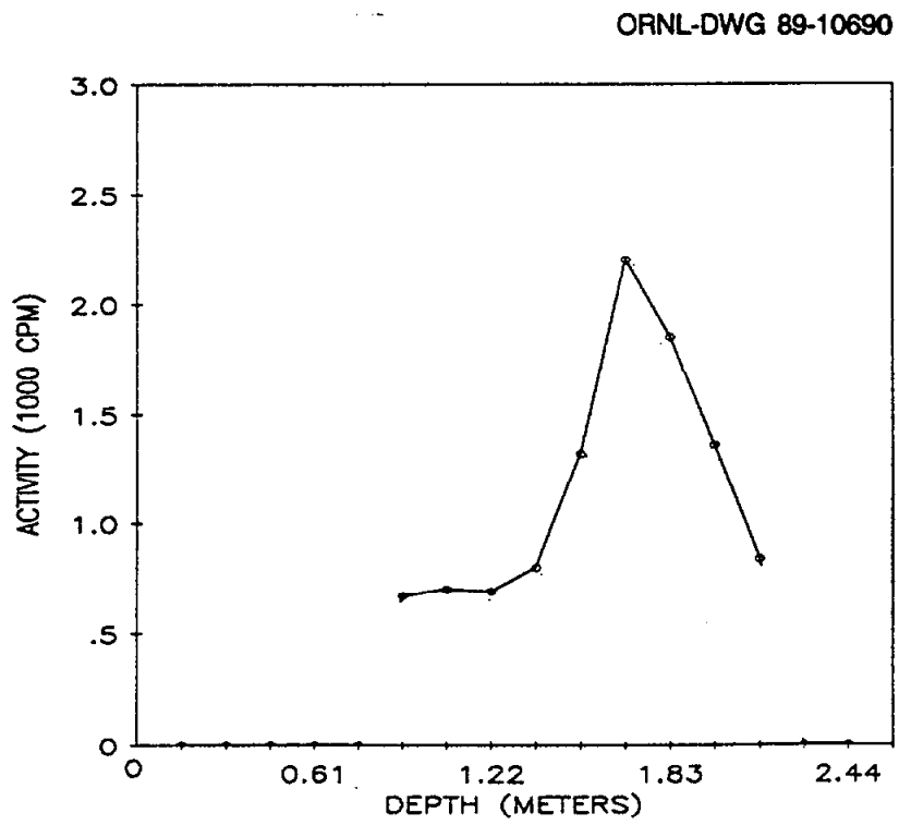
Fig. 9. Gamma profile for auger hole 12 (LJ061A12) at 80 Industrial Road, Lodi, New Jersey.
