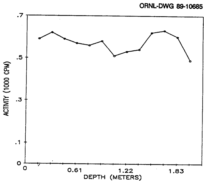
Fig. 4. Gamma profile for auger hole 3 (LJ061A3) at 80 Industrial Road, Lodi, New Jersey.
