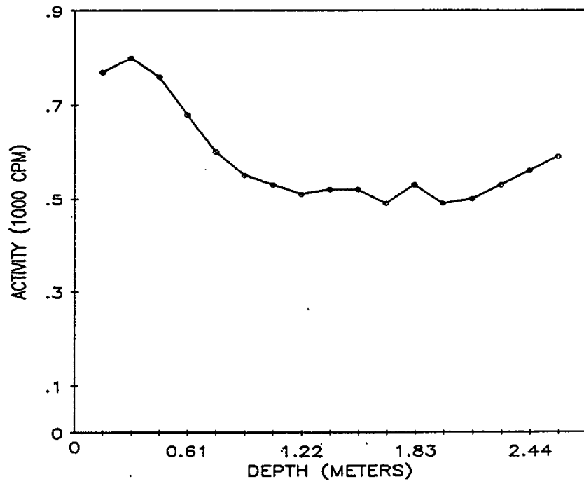
Fig. 6. Gamma profile for auger hole 5 (LJ061A5) at 80 Industrial Road, Lodi, New Jersey.
