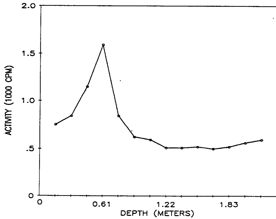
Fig. 7. Gamma profile for auger hole 8 (LJ061A8) at 80 Industrial Road, Lodi, New Jersey.
