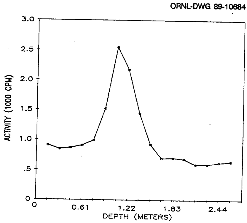
Fig. 3. Gamma profile for auger hole 2 (LJ061A2) at 80 Industrial Road, Lodi, New Jersey.
