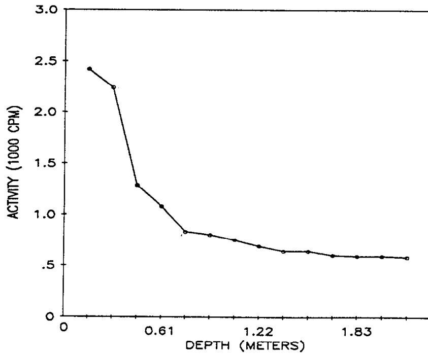
Fig. 5. Gamma profile for auger hole 4 (LJ061A4) at 80 Industrial Road, Lodi, New Jersey.
