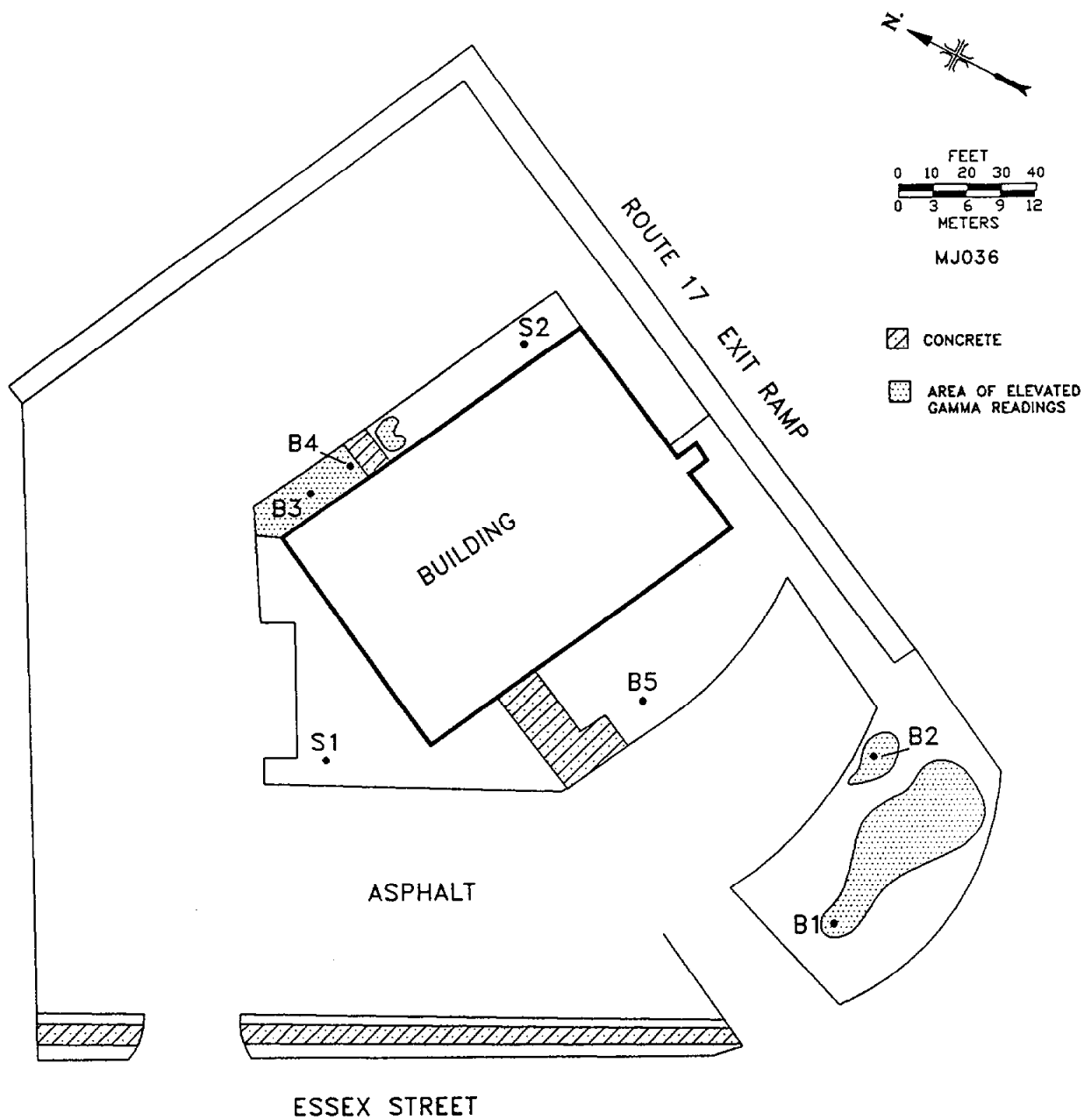
Fig. 2. Diagram showing locations of soil samples taken at Essex Street and State Route 17, Maywood, New Jersey (MJ036).
