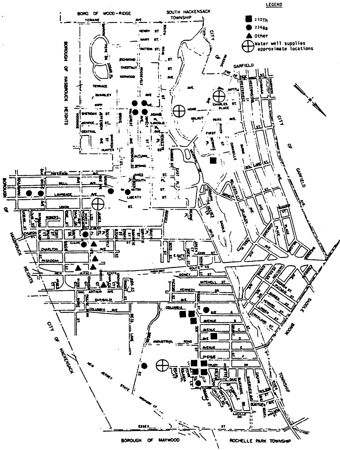
Fig. 1. Area surveyed during the mobile gamma scan of Lodi, New Jersey.
