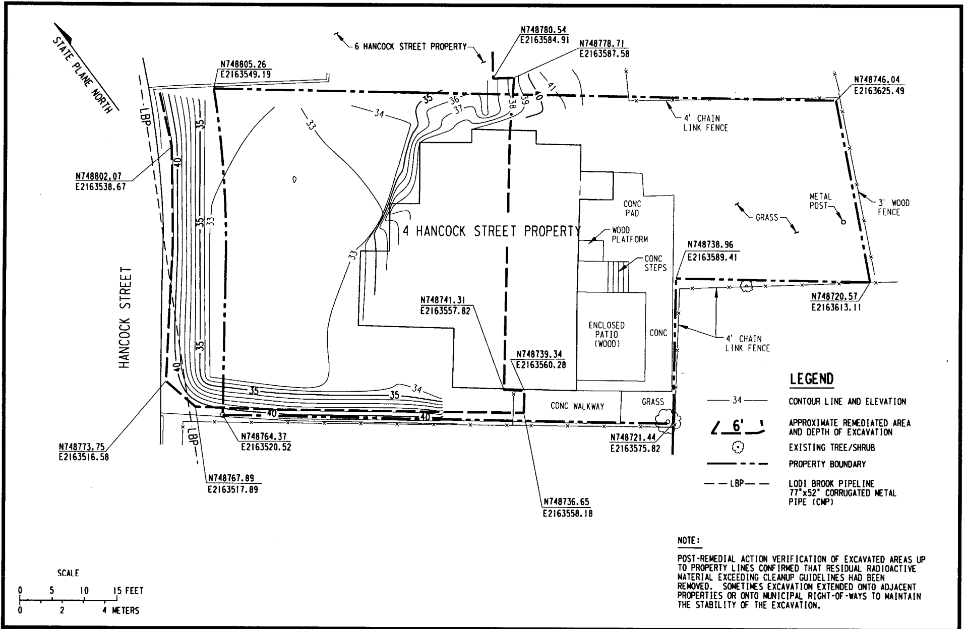
Figure 4-1 Areas of Excavation and Elevation Contours 4 Hancock Street
