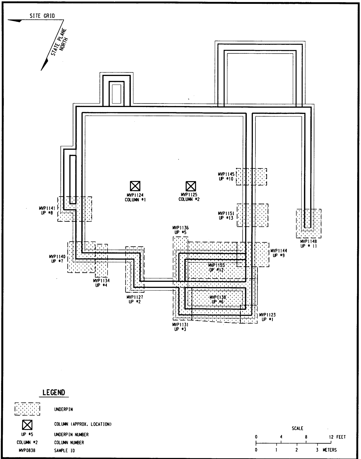
Figure 4-3 Areas of Underpin and Column Excavation and Post-Remedial Action Samples 4 Hancock Street
