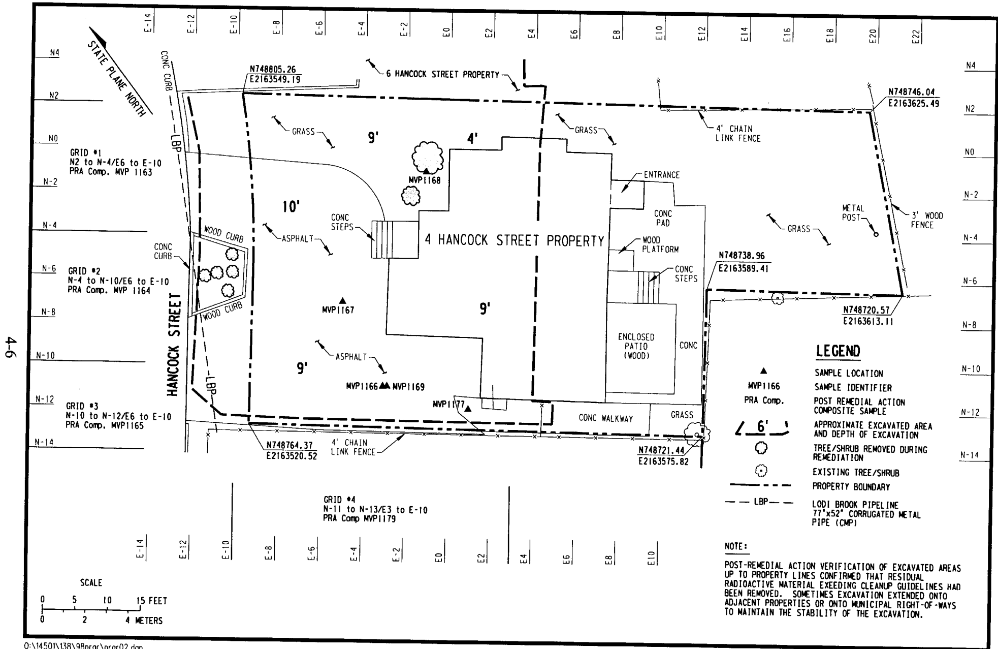
Figure 4-2 Areas of Excavation and Post-Remedial Action Samples 4 Hancock Street
