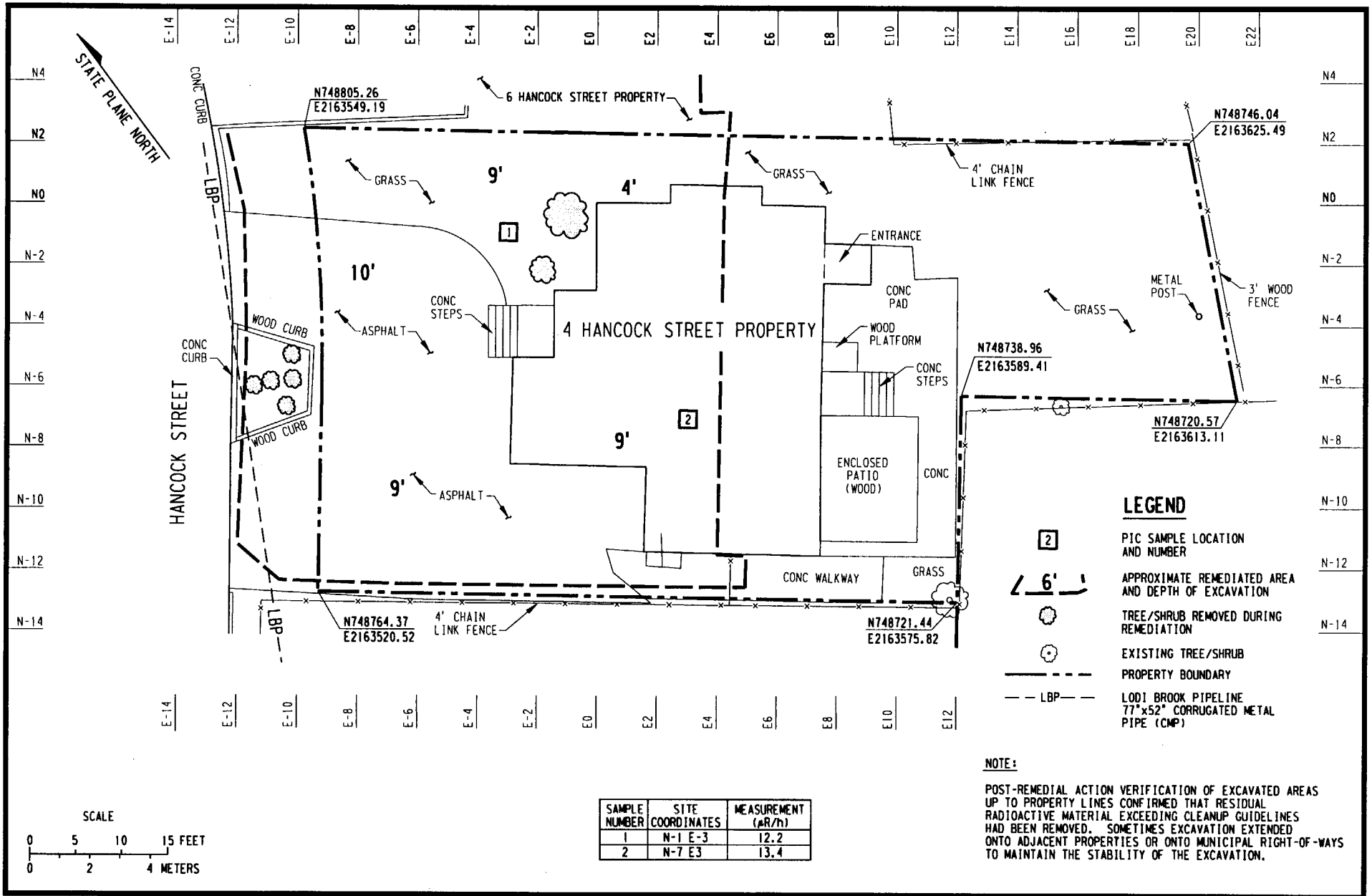
Figure 4-6 PIC Readings 4 Hancock Street
