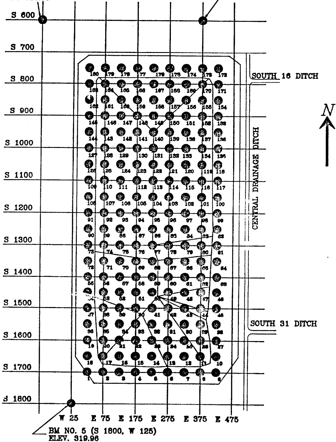
SURVEY GRID FOR THE NFSS WASTE CONTAINMENT STRUCTURE
