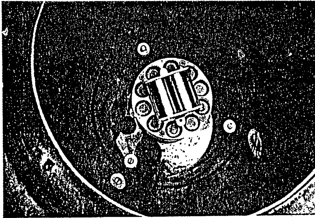
Fig. I-I. Soil sample holder on germanium-detector system.
