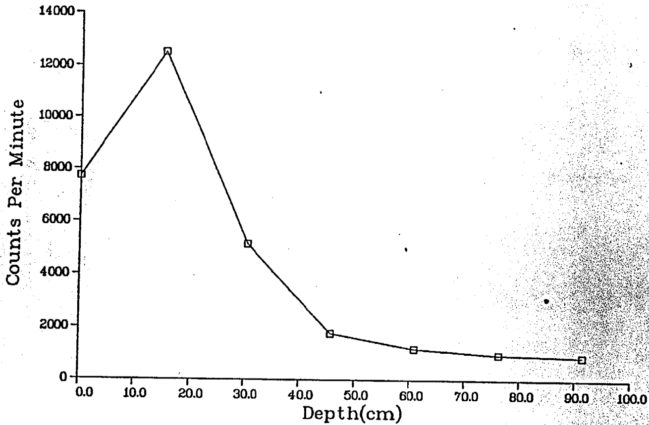
Fig. II-3. Gamma profile of core hole MJC36 (see Fig. 6)
