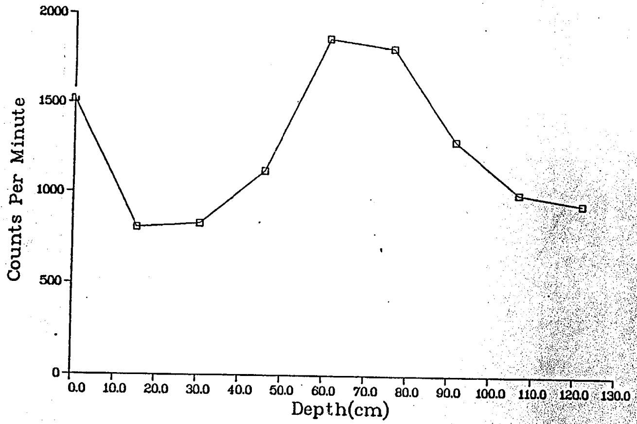
Fig. II-2. Gamma profile of core hole MJC35 (see Fig. 6)
