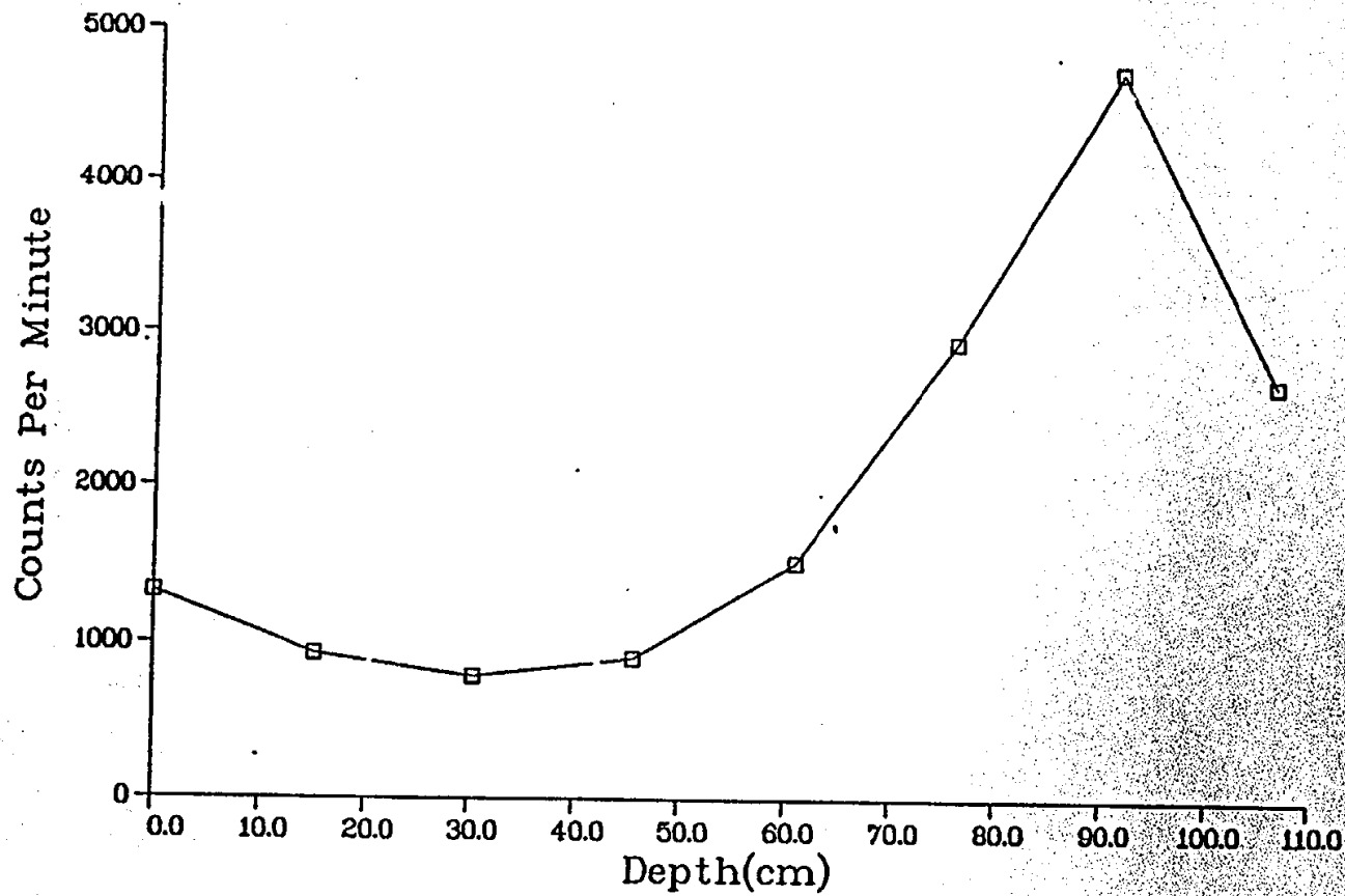
Fig. II-1, Gamma profile of core hole MJC34 (see Fig. 6)
