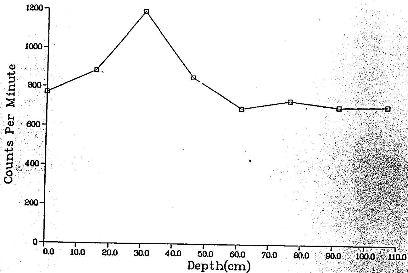
Fig. II-4. Gamma profile of core hole MJC37 (see Fig. 6)
