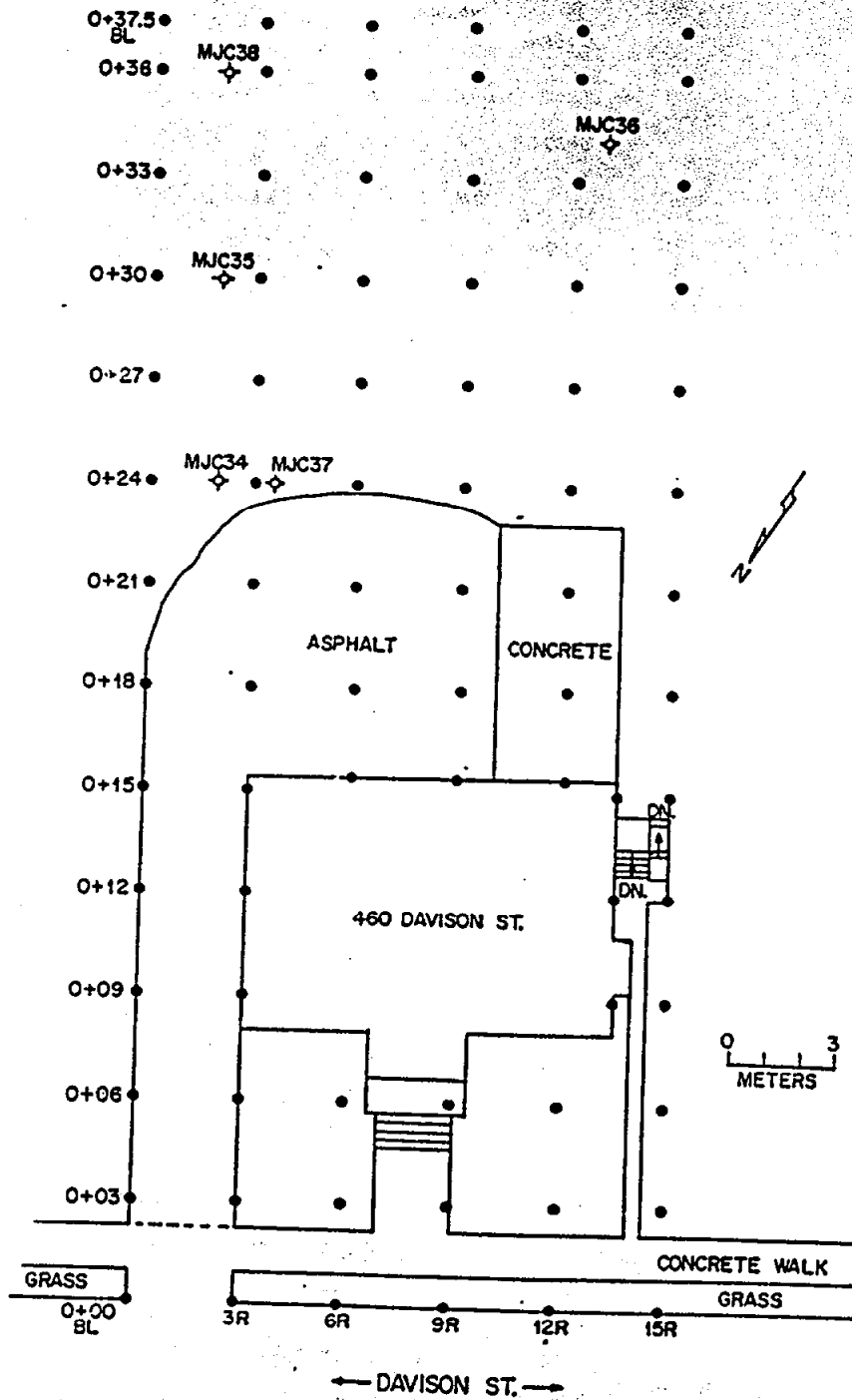
Fig. 6. Location of drill holes at 460 Davison Avenue
