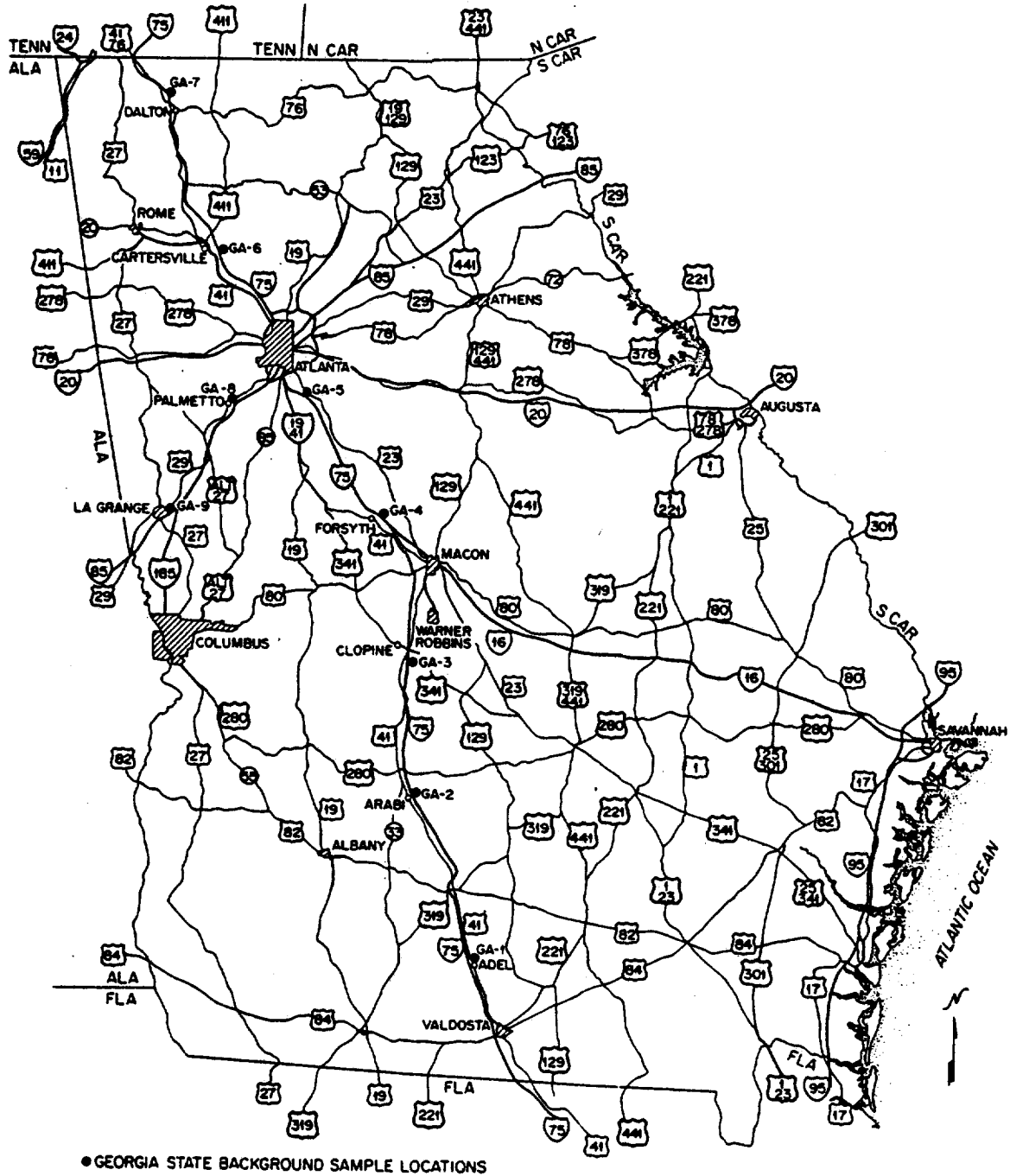
Fig. 10. Location of background samples and external gamma-ray exposure rate measurements in Georgia.
