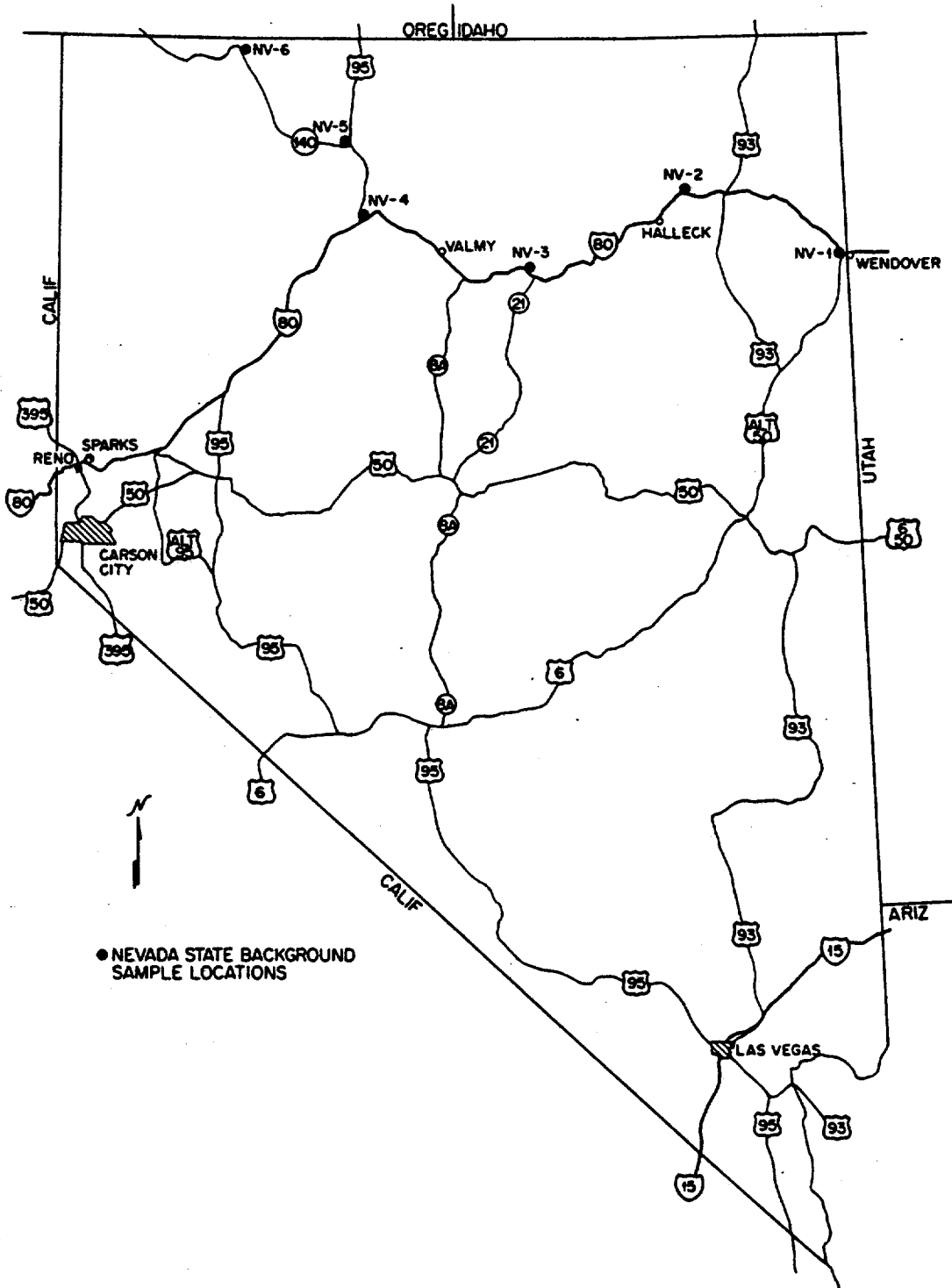
Fig. 20. Location of background samples and external gamma-ray exposure rate measurements in Nevada.
