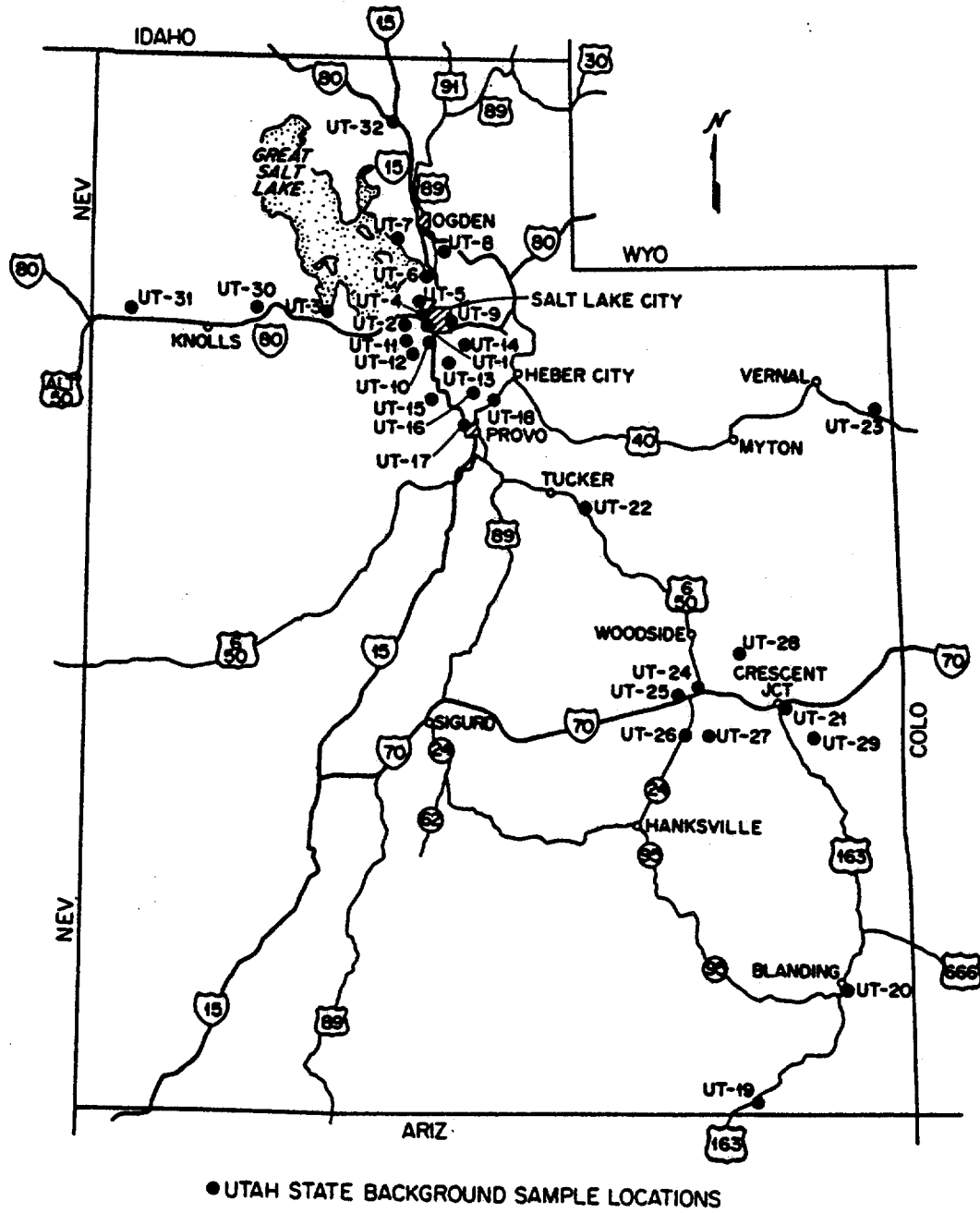
Fig. 30. Location of background samples and external gamma-ray exposure rate measurements in Utah.
