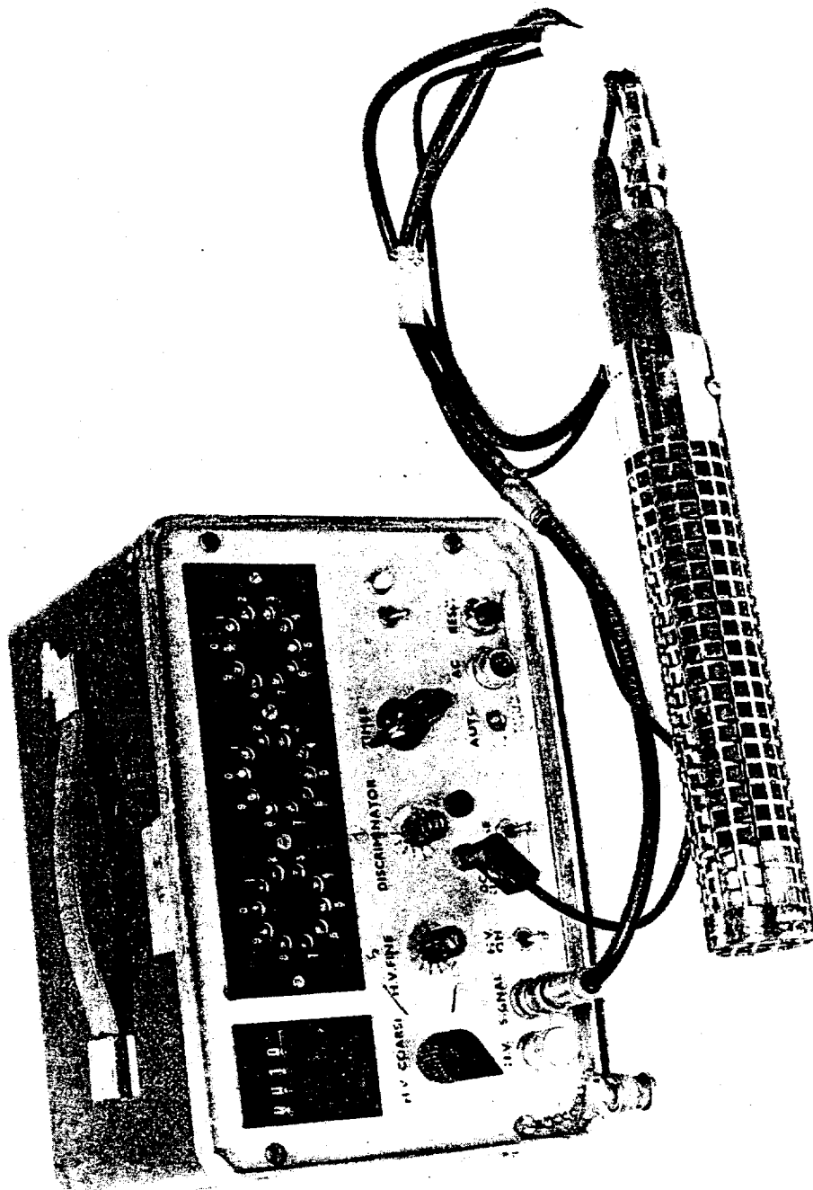
Fig. I-A. Glass-walled, organic-filled Geiger-Mueller (G-M) tube with a battery-powered portable scaler.
