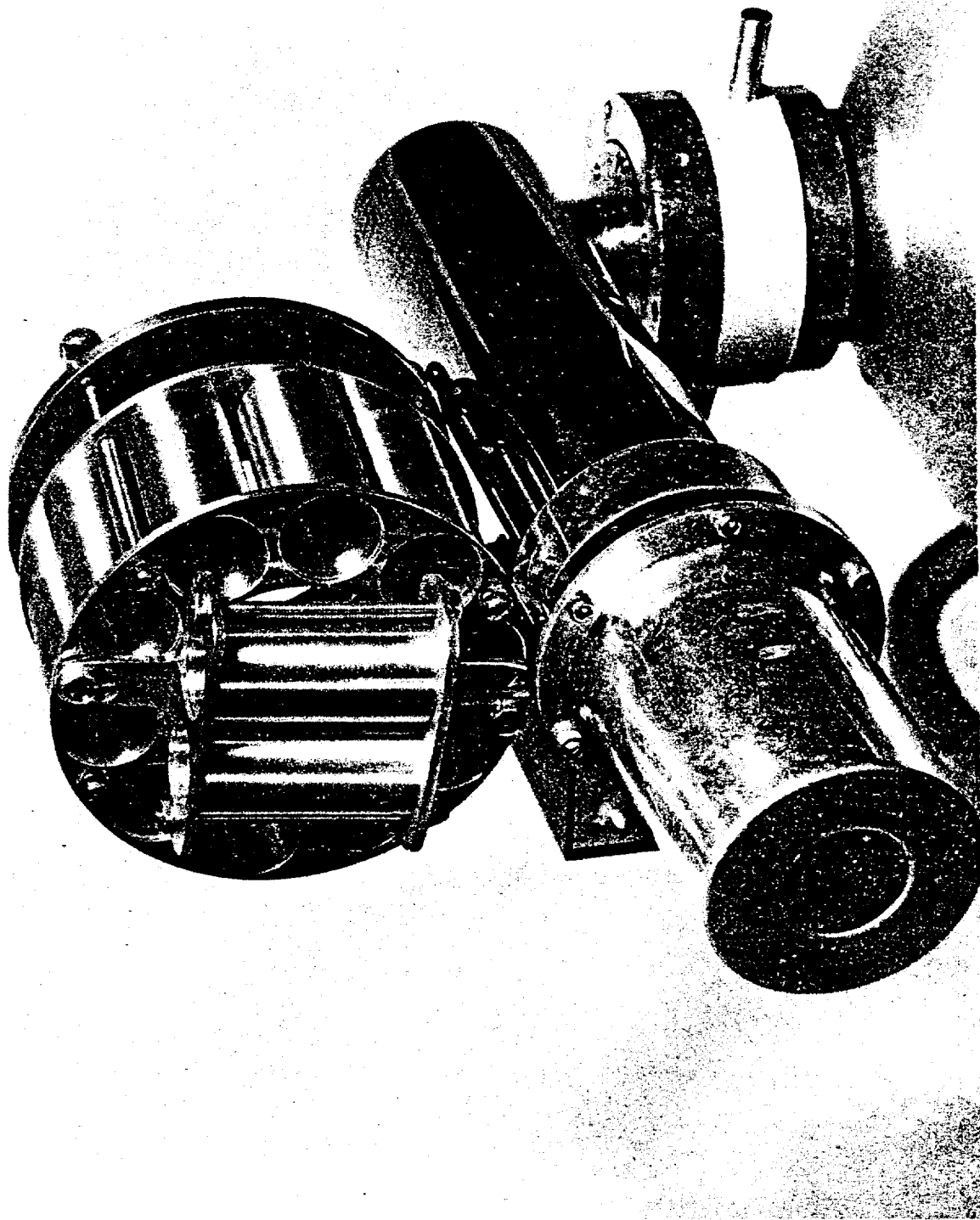
Fig. II-A. Soil sample holder above the Ge(Li) detector.
