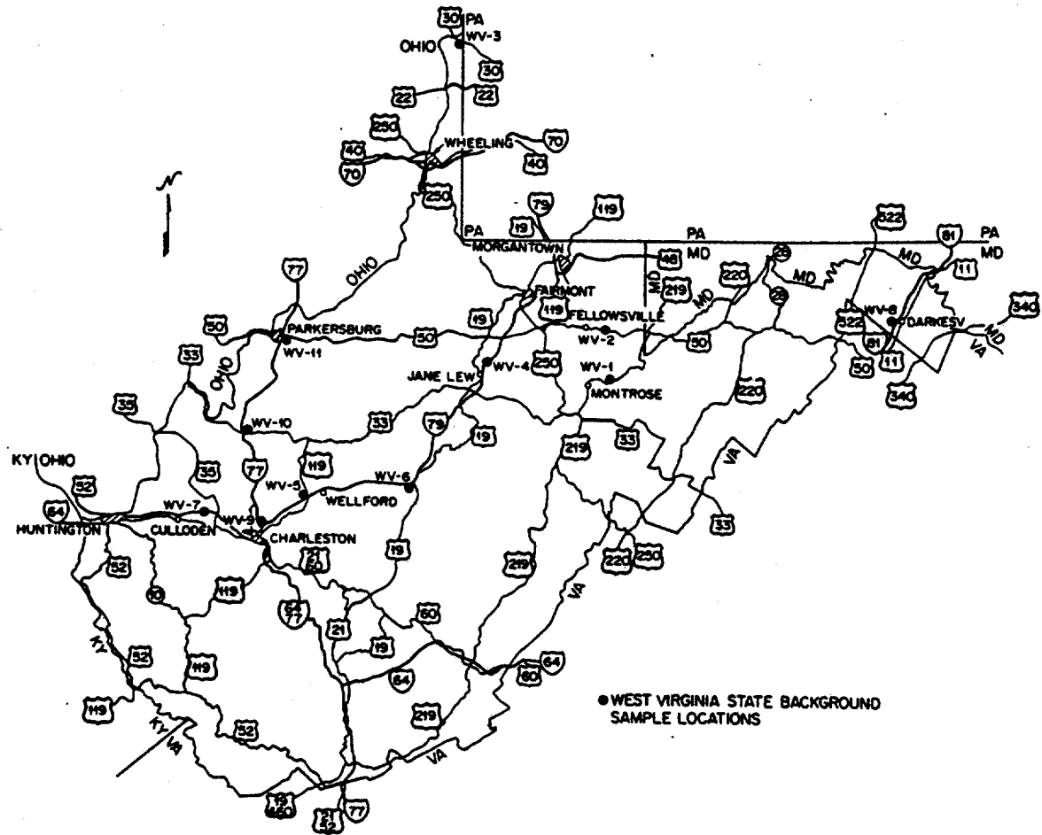
Fig. 32. Location of background samples and external gamma-ray exposure rate measurements in West Virginia.
