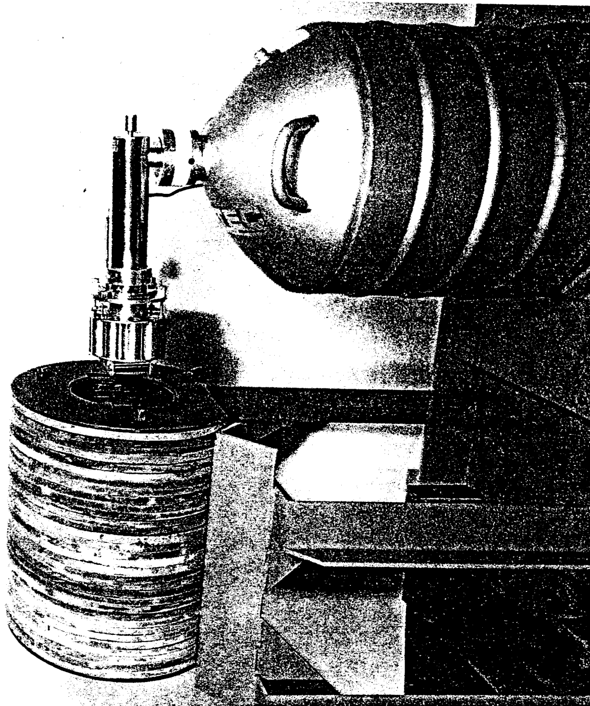
Fig. II-B. Soil sample holder attached to Ge(Li) detector.
