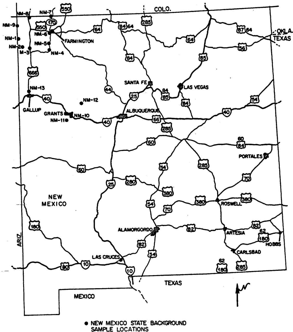
Fig. 22. Location of background samples and external gamma-ray exposure rate measurements in New Mexico.
