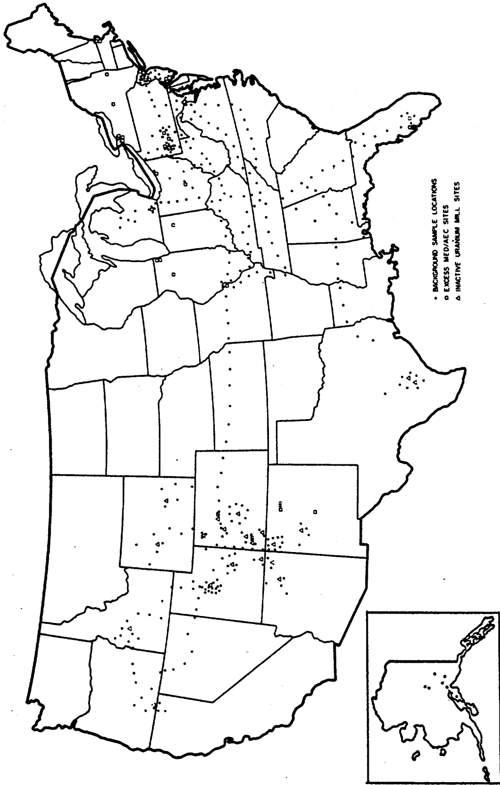
Fig. 1. Location of background soil samples and external gamma-ray exposure rate measurements in the United States.
