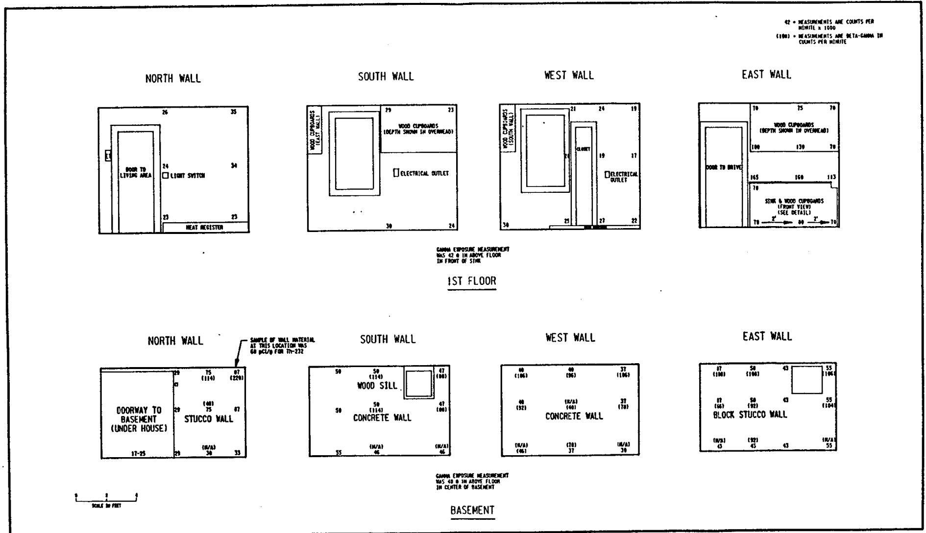
FIGURE 3 KITCHEN AS-BUILT, 90 AVENUE "C"
