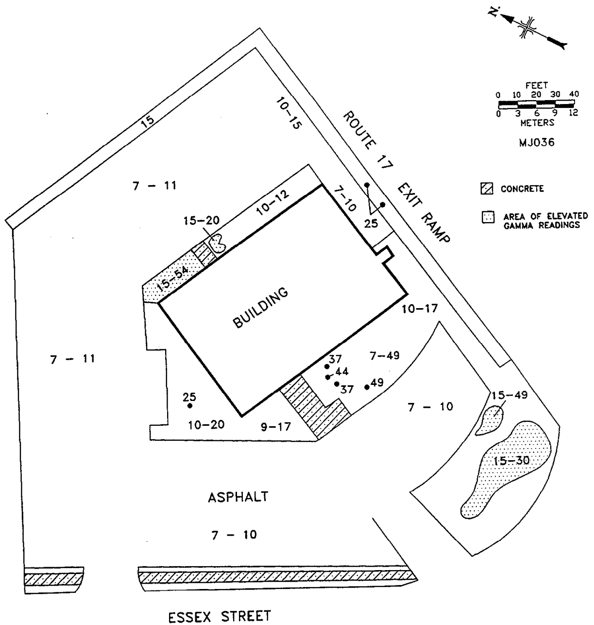
Fig. 1. Gamma radiation levels ( \mu\text{R/h} ) measured on the surface at Essex Street and State Route 17, Maywood, New Jersey (MJ036).
