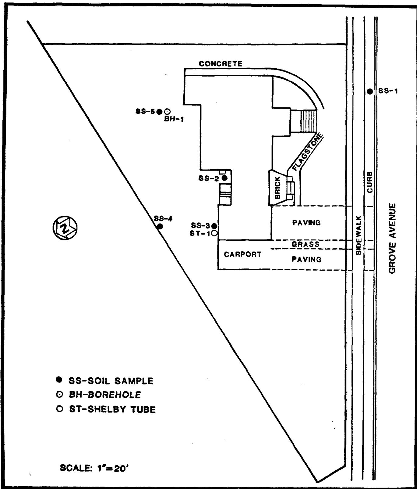
FIGURE 3-2 LOCATIONS OF SURFACE SOIL SAMPLES, BOREHOLE, AND SHELBY TUBE CORE SAMPLE AT 10 GROVE AVENUE
